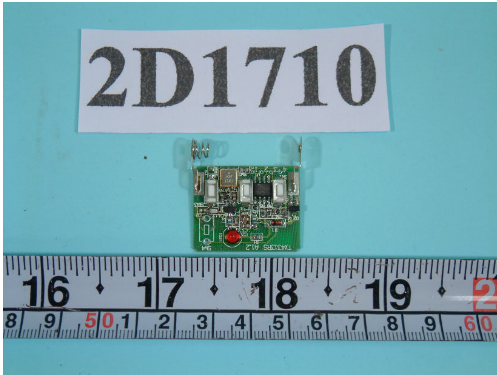
FRONT SIDE OF MAIN BOARD (FOR THREE BUTTON)
