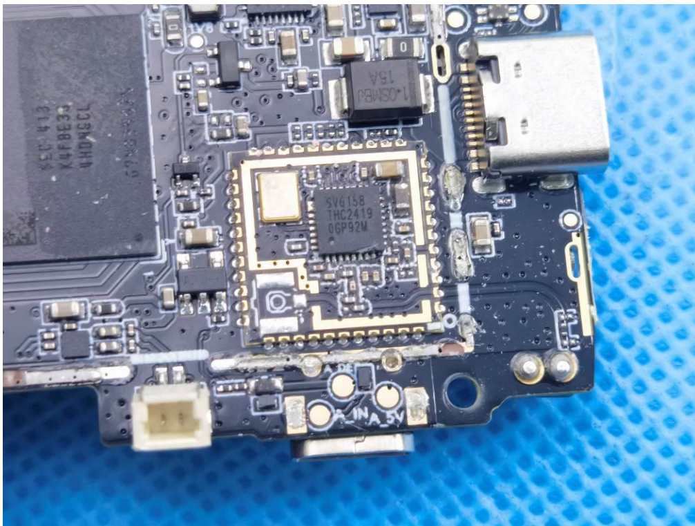
INTERNAL VIEW OF EUT (FIGURE 134)
