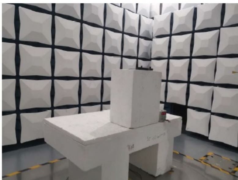
Radiated Spurious Emissions Test View (90-100GHz)
