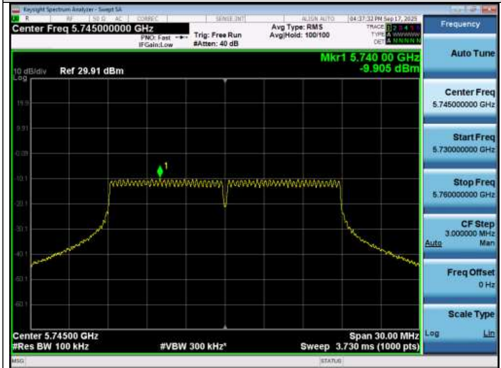
Test_Graph_802.11n20_ANT1_5745_MCS0_PSD
