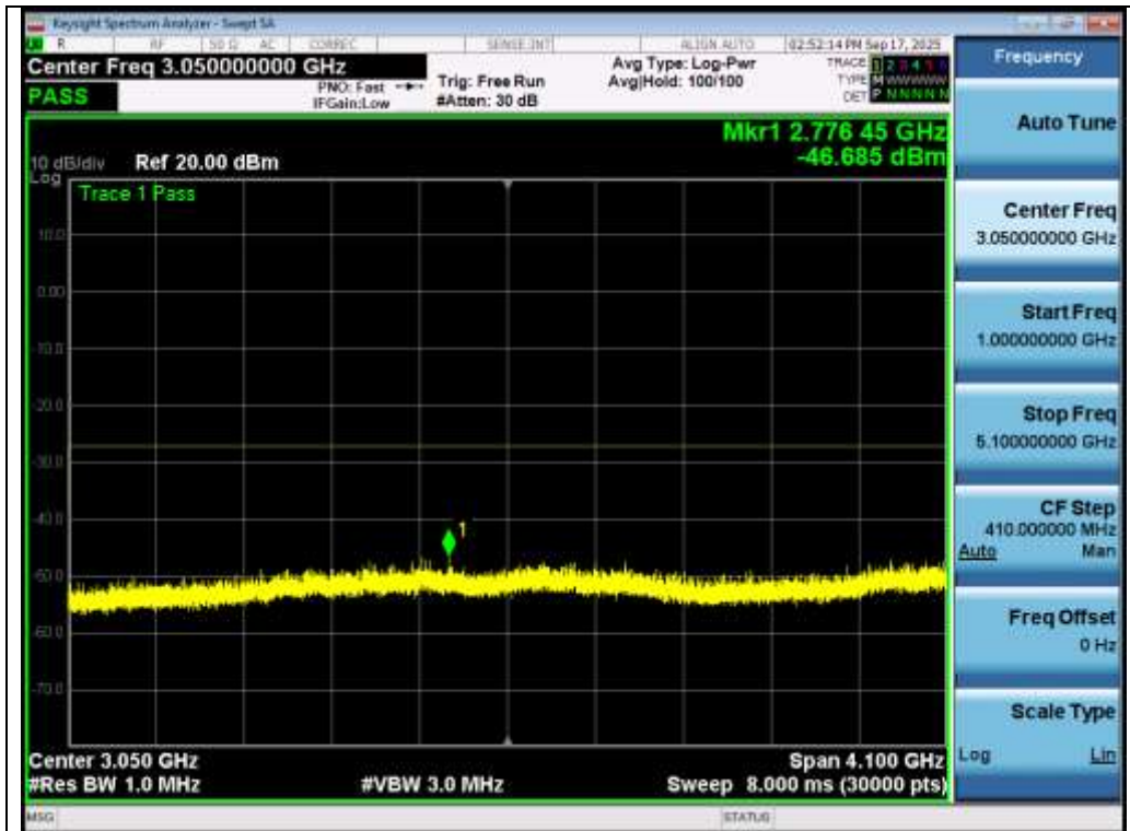
Test_Graph_802.11n40_ANT1_5230_MCS0_Frequency Band 2
