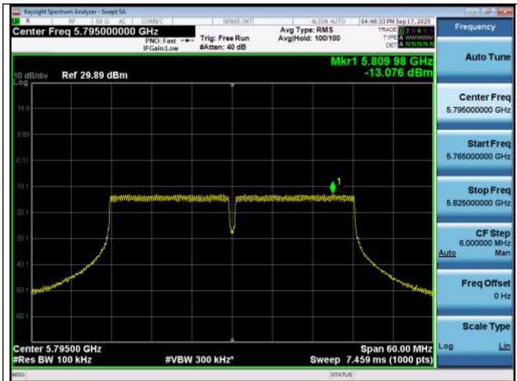
Test_Graph_802.11ac40_ANT1_5795_MCS0_PSD
