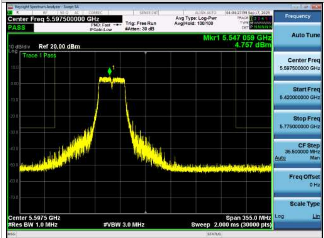
Test_Graph_802.11n40_ANT1_5550_MCS0_Frequency Band 3
