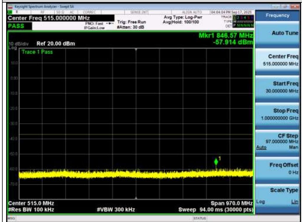
Test_Graph_802.11n40_ANT1_5550_MCS0_Frequency Band 1
