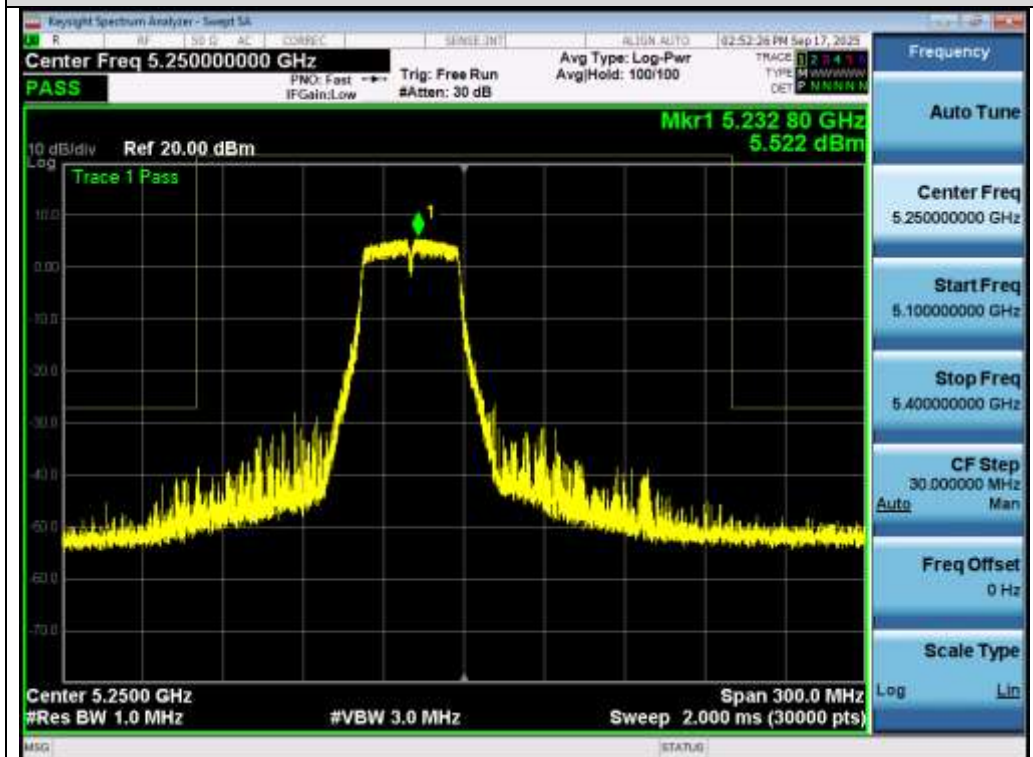
Test_Graph_802.11n40_ANT1_5230_MCS0_Frequency Band 3
