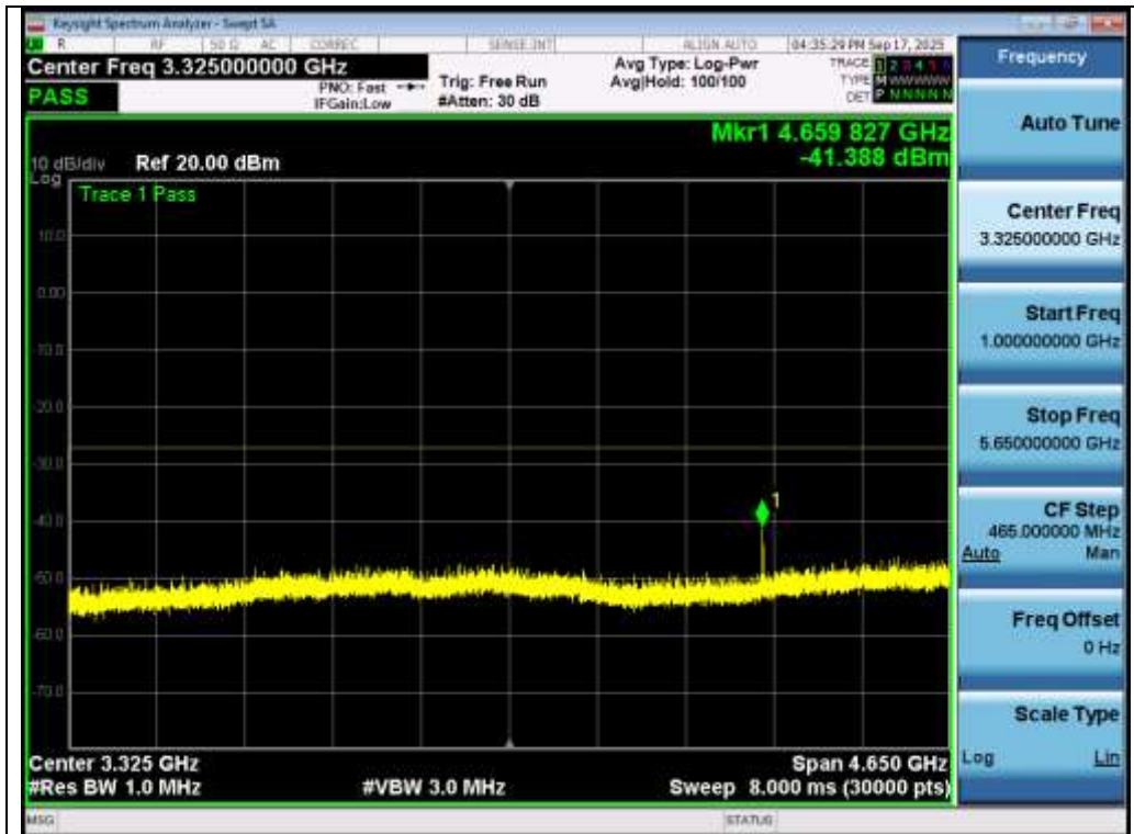
Test_Graph_802.11a_ANT1_5825_6Mbps_Frequency Band2
