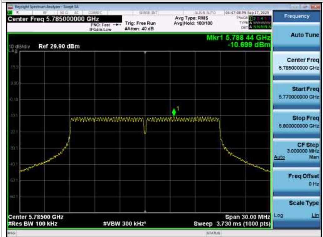
Test_Graph_802.11ac20_ANT1_5785_MCS0_PSD
