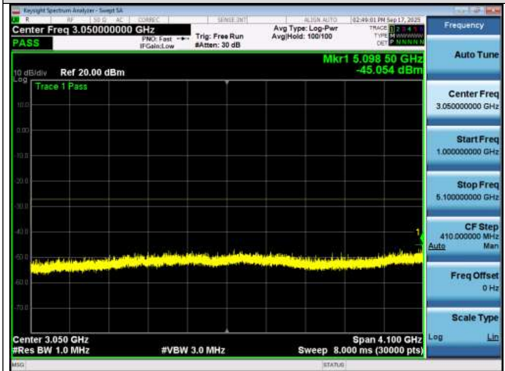
Test_Graph_802.11n40_ANT1_5190_MCS0_Frequency Band 2
