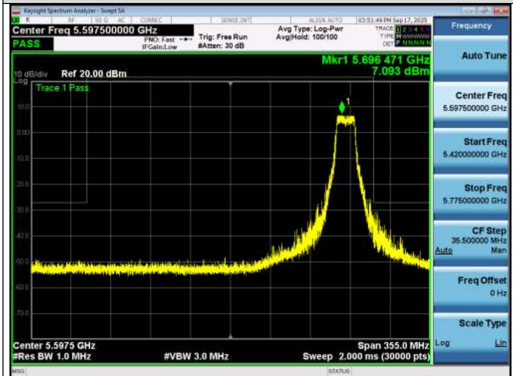
Test_Graph_802.11a_ANT1_5700_6Mbps_Frequency Band 3
