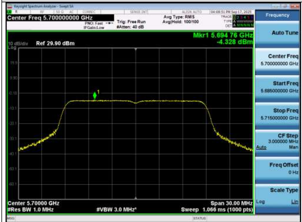
Test_Graph_802.11ac20_ANT1_5700_MCS0_PSD
