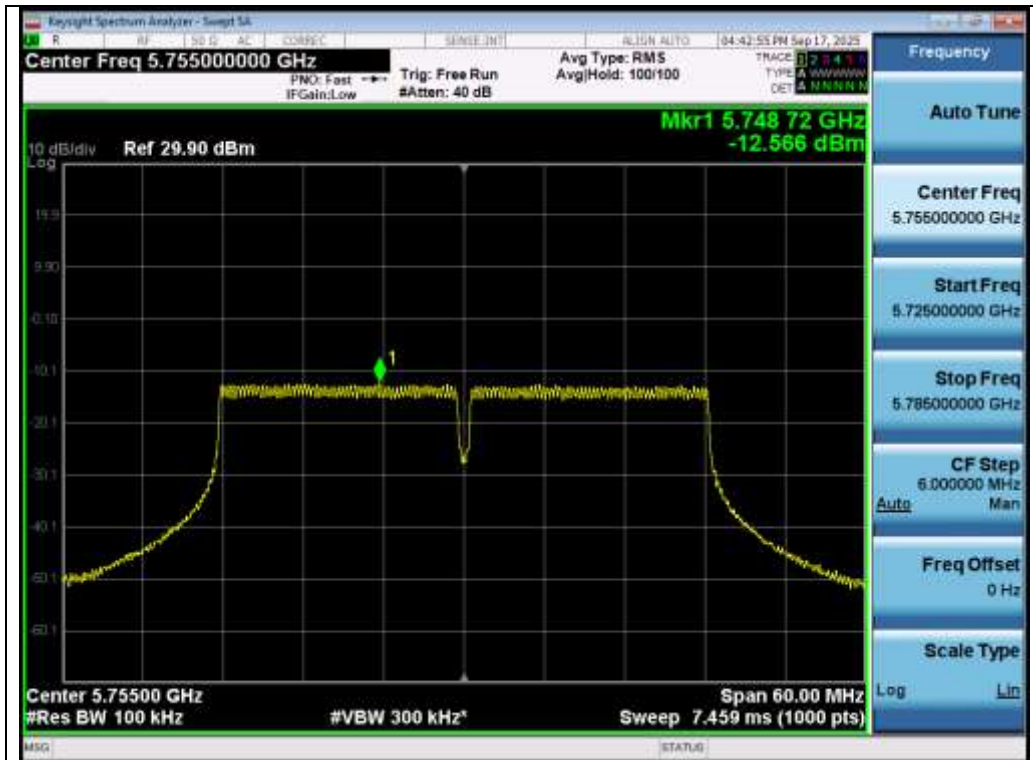
Test_Graph_802.11n40_ANT1_5755_MCS0_PSD
