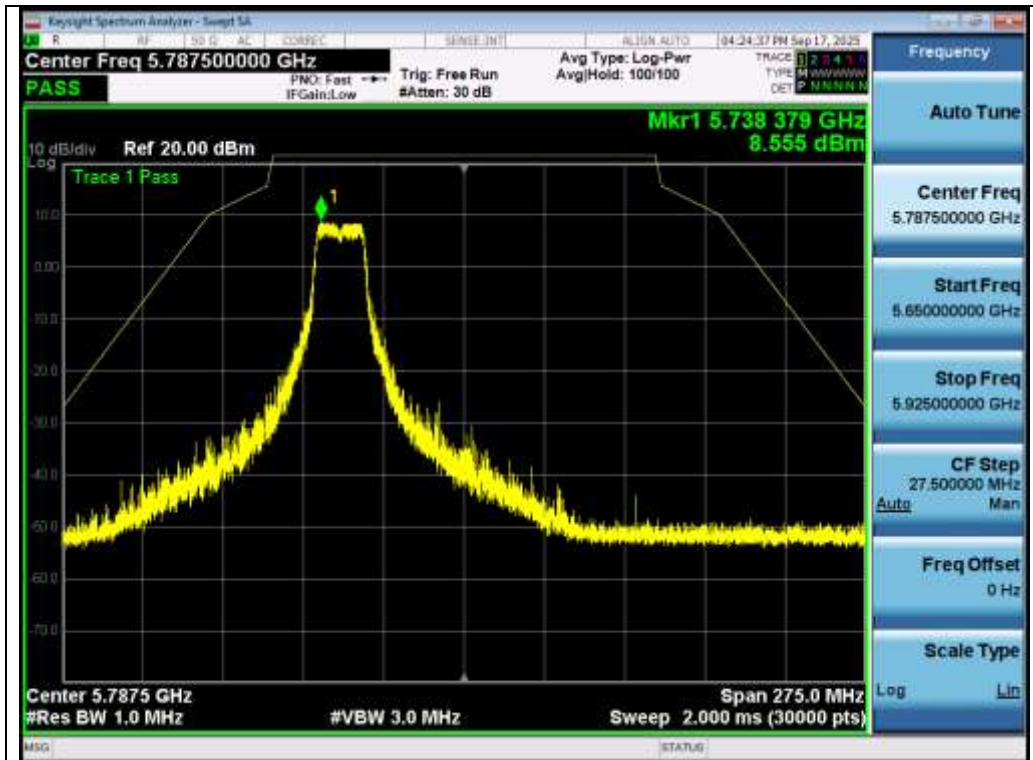
Test_Graph_802.11a_ANT1_5745_6Mbps_Frequency Band3
