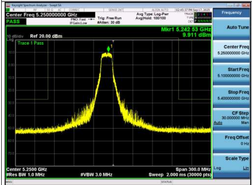
Test_Graph_802.11a_ANT1_5240_6Mbps_Frequency Band 3
