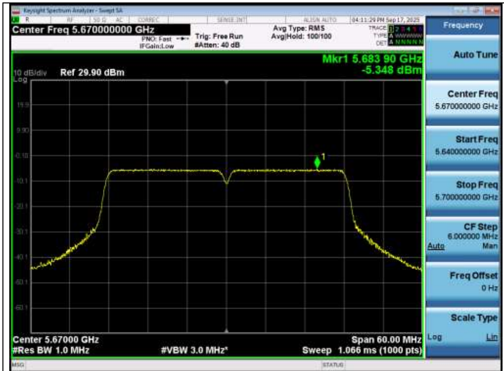
Test_Graph_802.11ac40_ANT1_5670_MCS0_PSD
