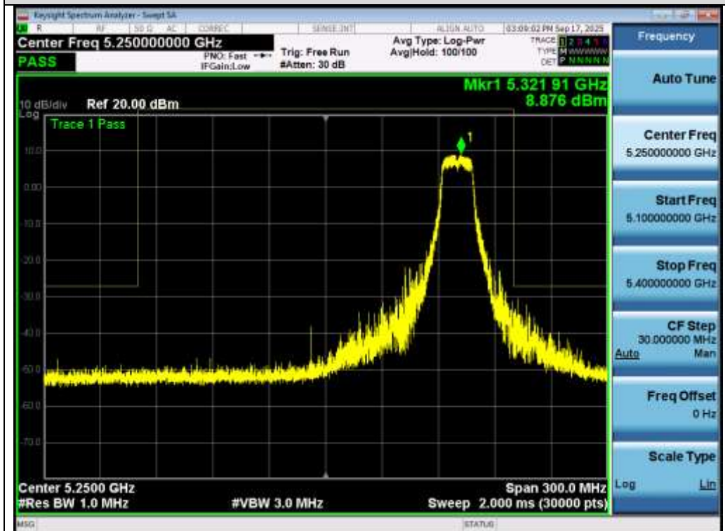
Test_Graph_802.11a_ANT1_5320_6Mbps_Frequency Band 3
