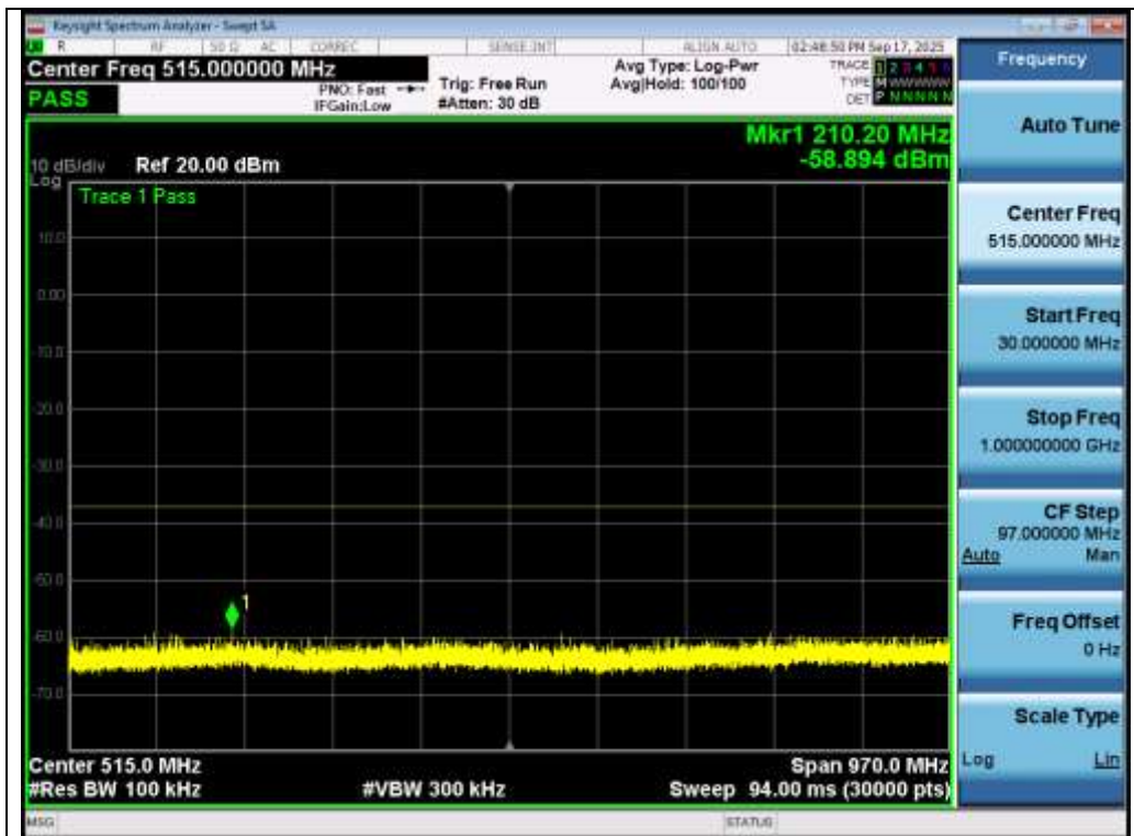
Test_Graph_802.11n40_ANT1_5190_MCS0_Frequency Band 1
