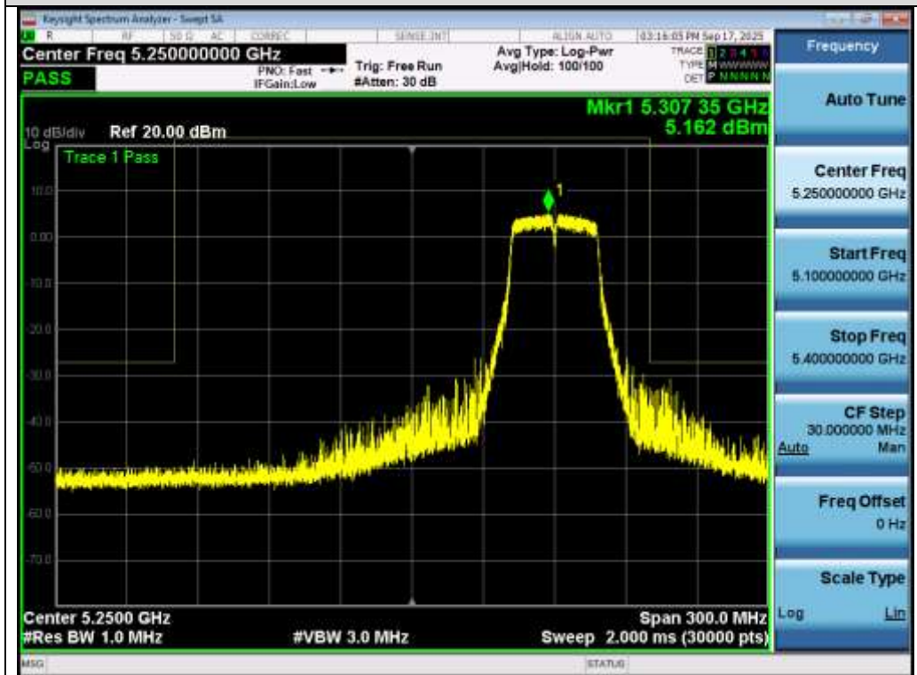
Test_Graph_802.11n40_ANT1_5310_MCS0_Frequency Band 3
