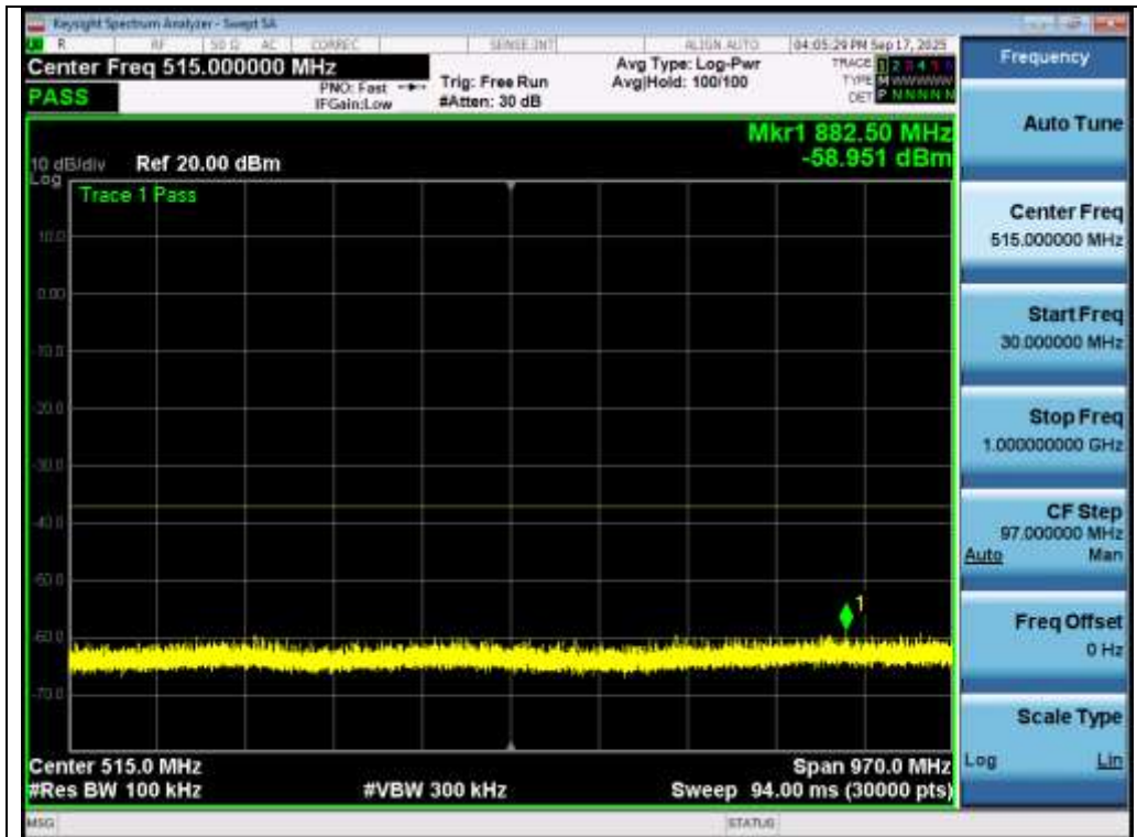
Test_Graph_802.11n40_ANT1_5670_MCS0_Frequency Band 1
