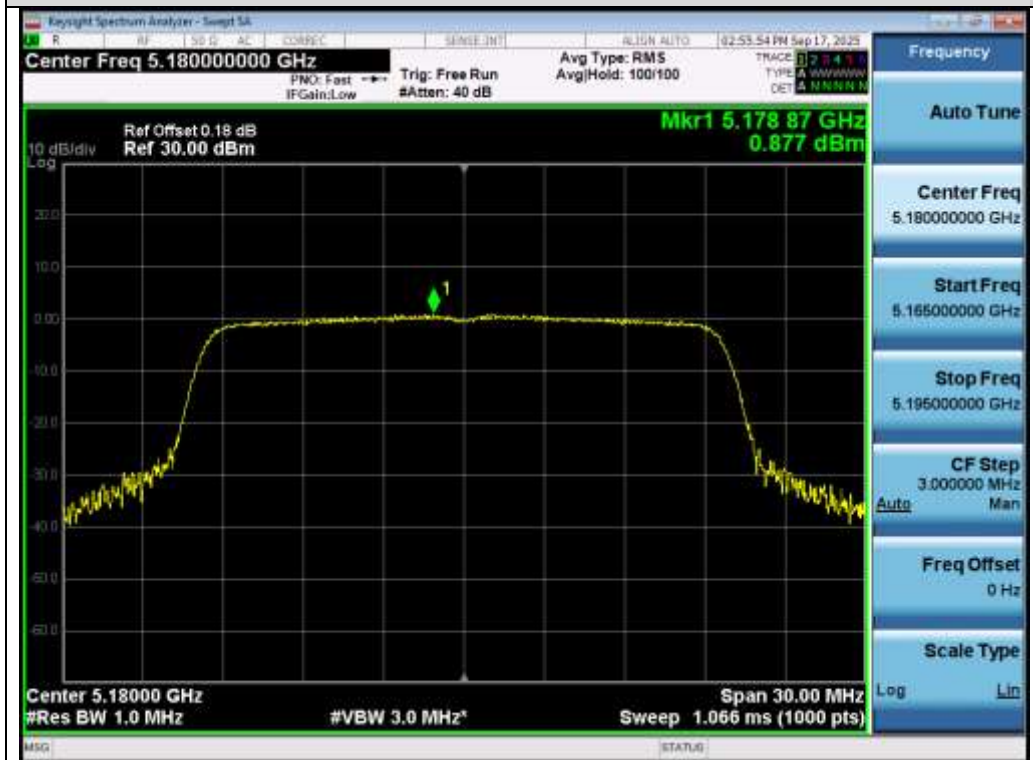
Test_Graph_802.11ax20_ANT1_5180_MCS0_PSD
