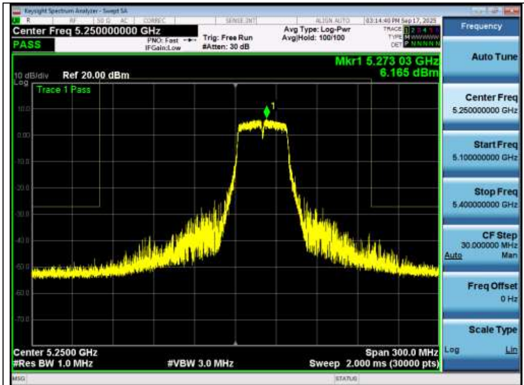
Test_Graph_802.11n40_ANT1_5270_MCS0_Frequency Band 3
