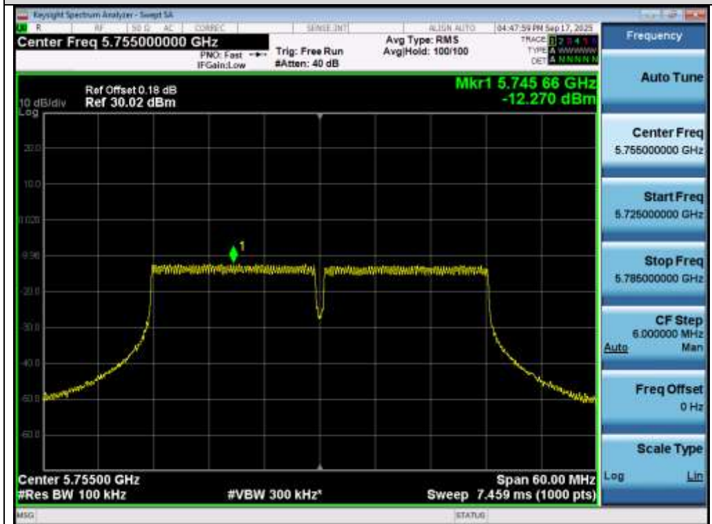
Test_Graph_802.11ac40_ANT1_5755_MCS0_PSD
