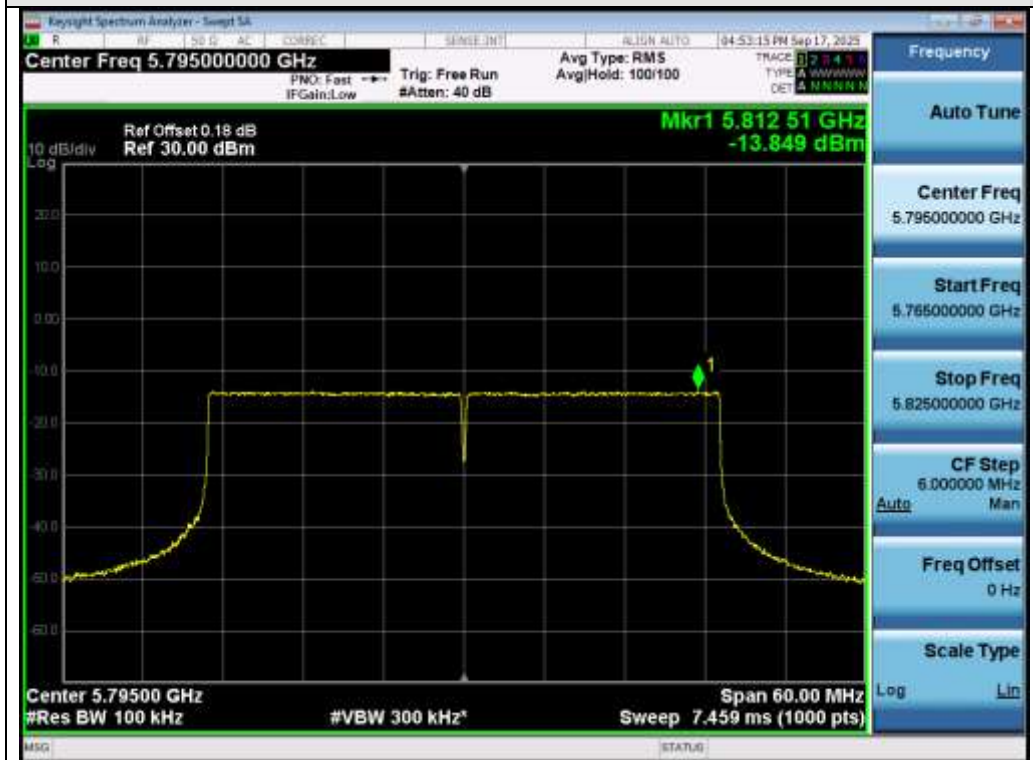
Test_Graph_802.11ax40_ANT1_5795_MCS0_PSD
