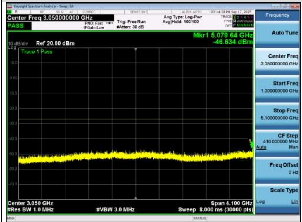
Test_Graph_802.11n40_ANT1_5270_MCS0_Frequency Band 2
