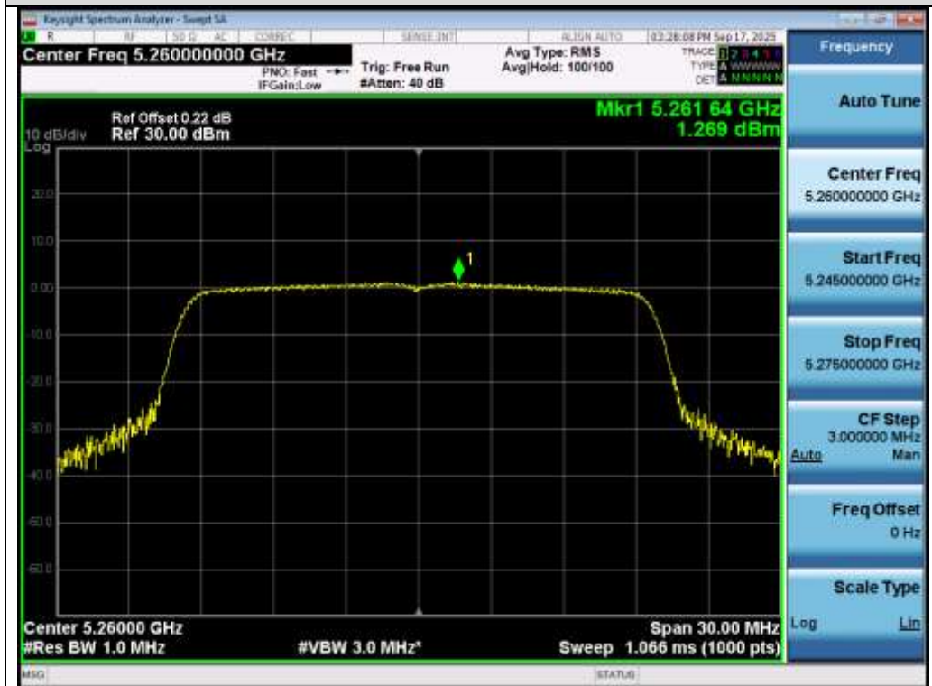
Test_Graph_802.11ax20_ANT1_5260_MCS0_PSD
