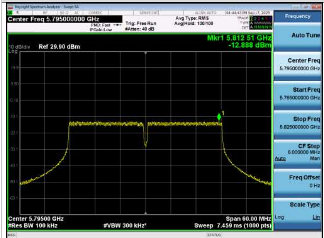
Test_Graph_802.11n40_ANT1_5795_MCS0_PSD
