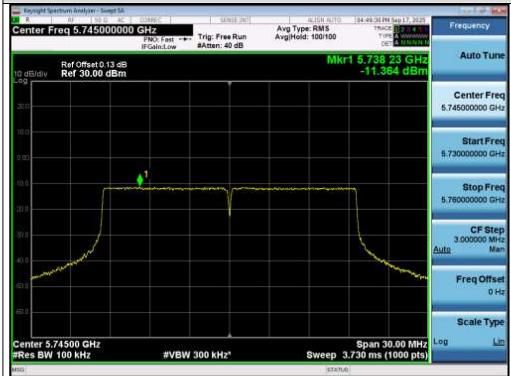
Test_Graph_802.11ax20_ANT1_5745_MCS0_PSD
