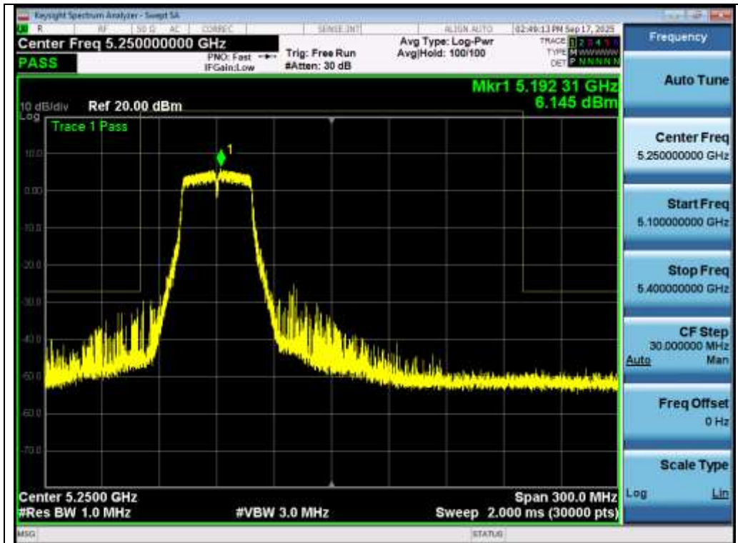
Test_Graph_802.11n40_ANT1_5190_MCS0_Frequency Band 3
