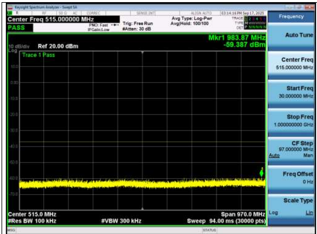
Test_Graph_802.11n40_ANT1_5270_MCS0_Frequency Band 1
