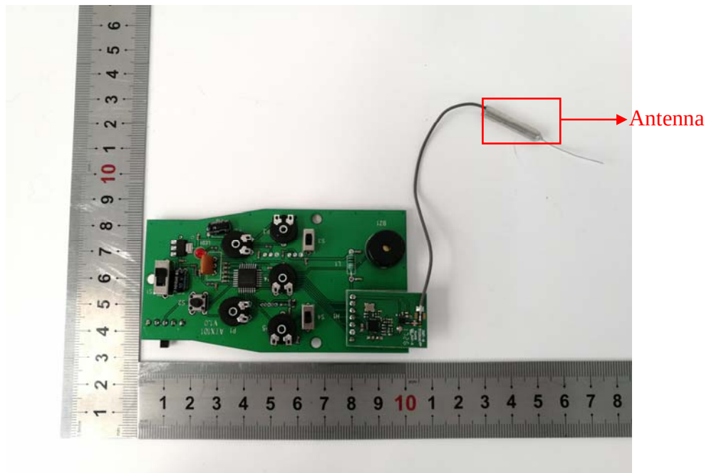
EUT – Module Top View
