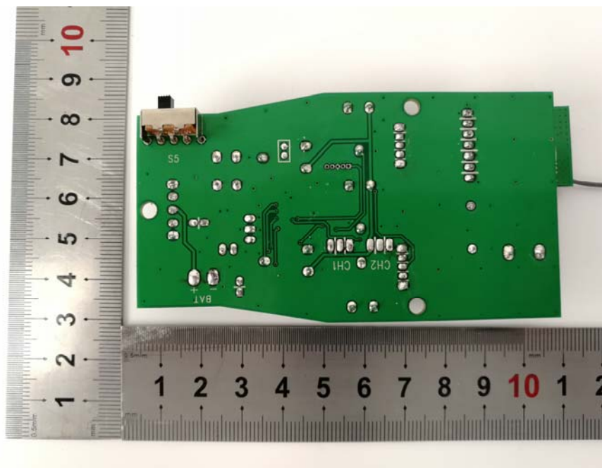
EUT – PCB Bottom View
