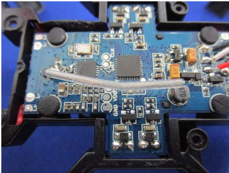
EUT –Remote Receiver Antenna View
