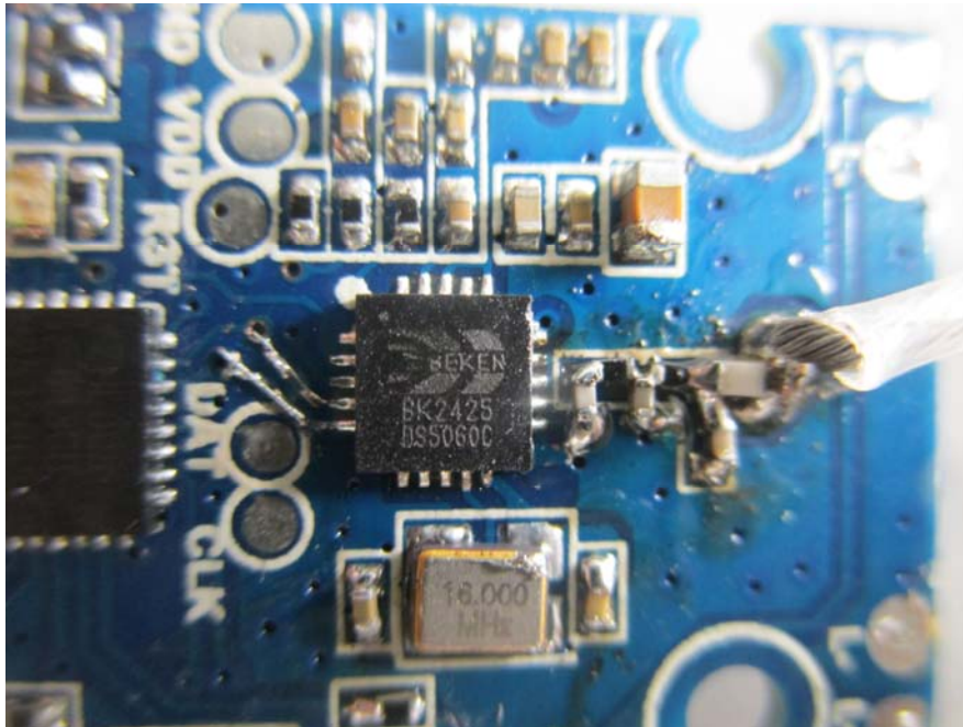
EUT –Remote Receiver Chip View
