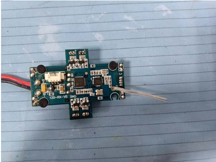
EUT – 2.4G Radio (only receive) Antenna
