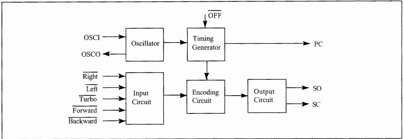
Block Diagram of 27.145 Mhz and 49.860 Mhz Transmitter
