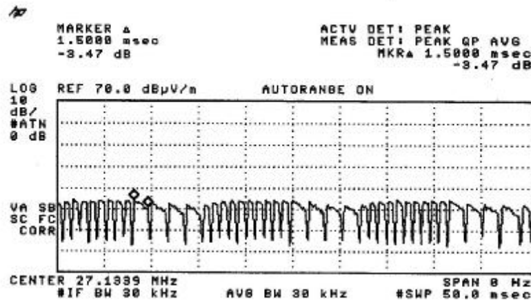
Figure C [Short Pulse]
