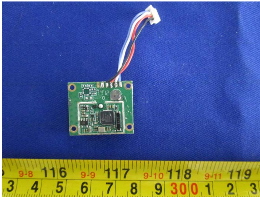
EUT – Subboard Unshielded View
