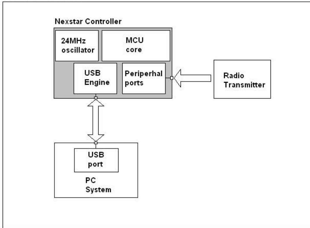
Nexstar Block Diagram
