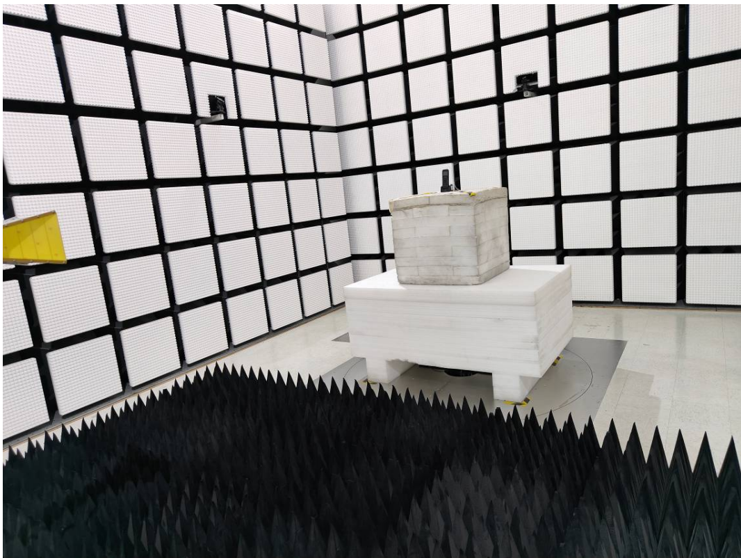
Radiated Emission Above 1G View
