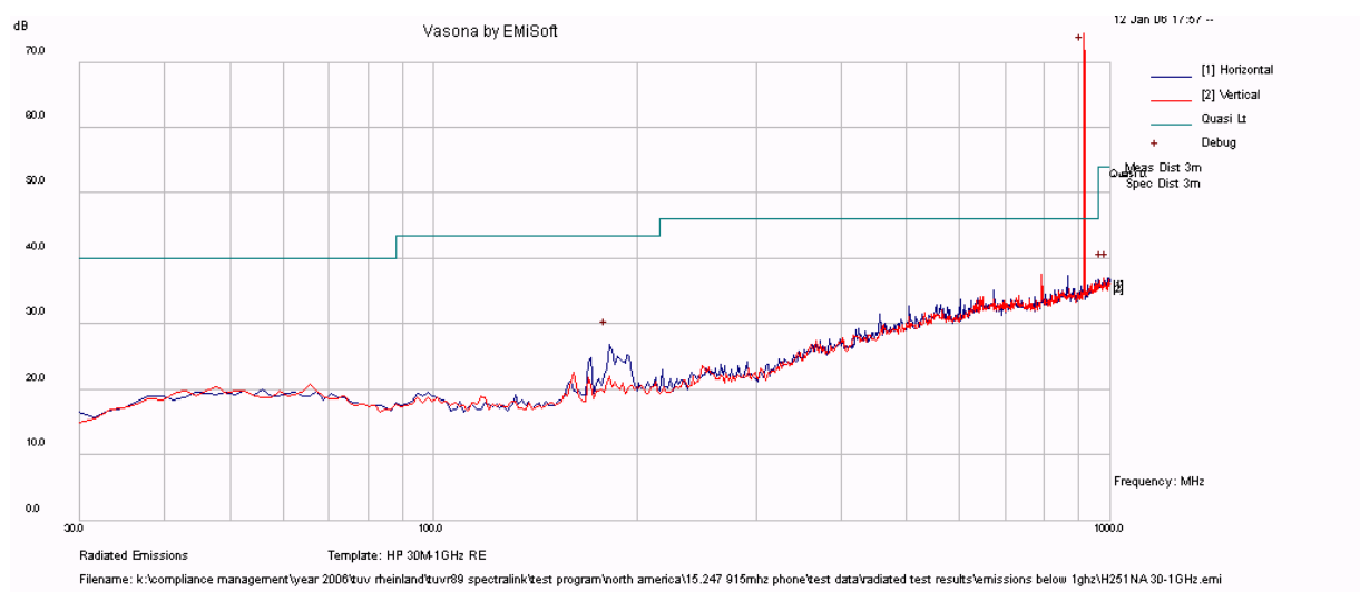
Plot 25 Radiated Emissions Below 1 GHz for EUT and H251NA Head Set
