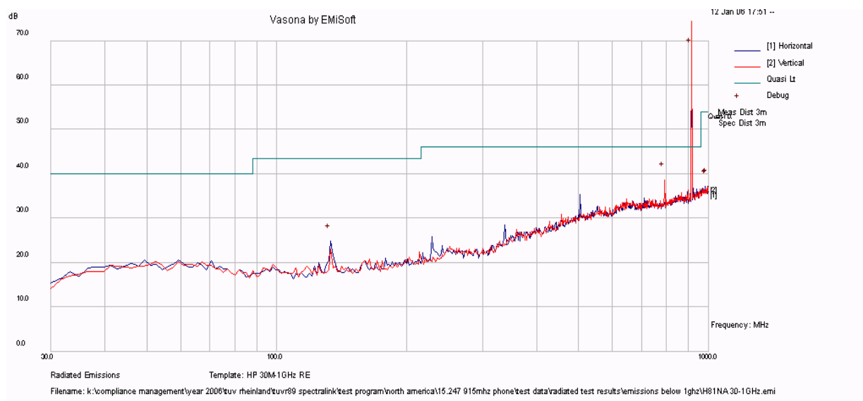
Plot 23 Radiated Emissions Below 1 GHz for EUT and H81NA Head Set
