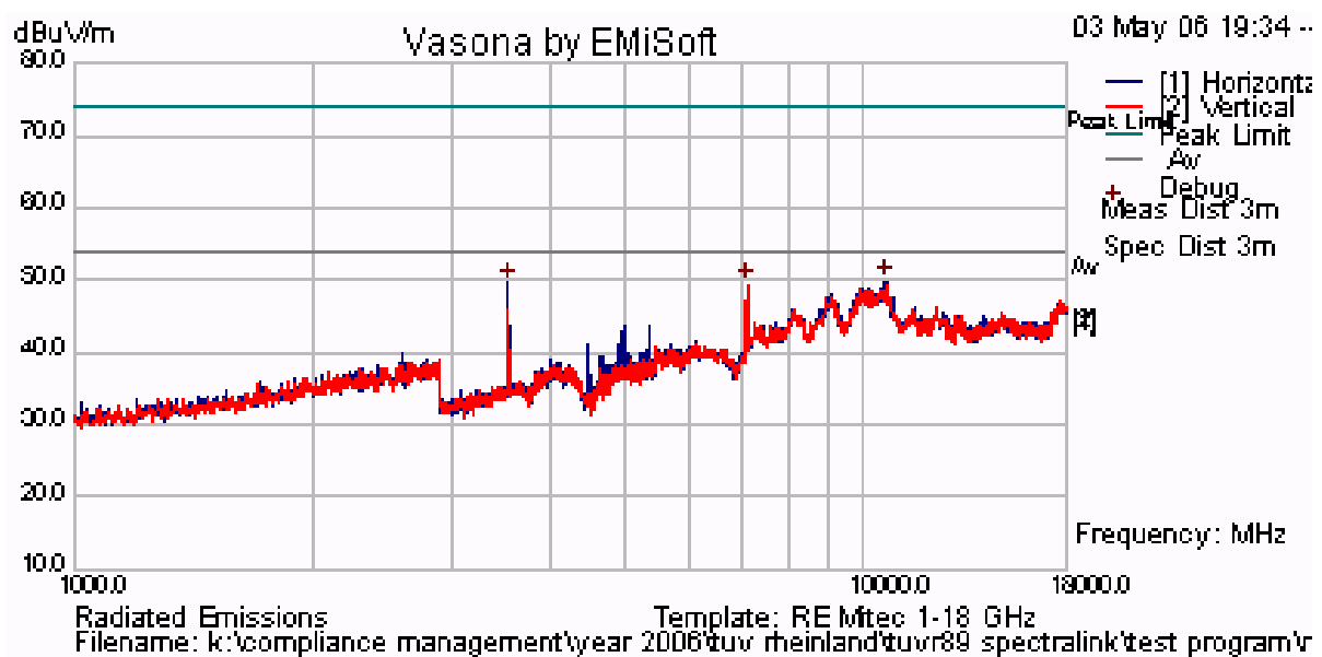
Plot 23 Radiated Emissions for 5,320 MHz
