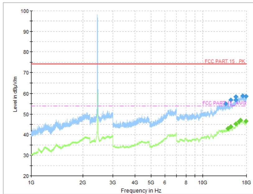
Fig.53 Radiated Spurious Emission (802.11n HT20, CH6, 1 GHz-18 GHz, MIMO)
