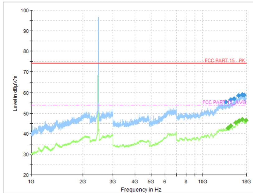
Fig.54 Radiated Spurious Emission (802.11n HT20, CH11, 1 GHz-18 GHz, MIMO)
