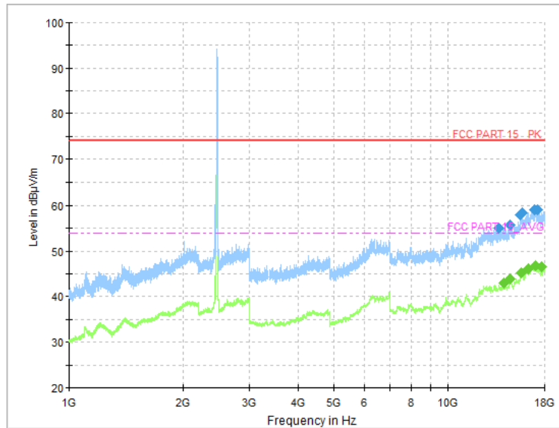
Fig.46 Radiated Spurious Emission (802.11n HT20, CH11, 1 GHz-18 GHz)
