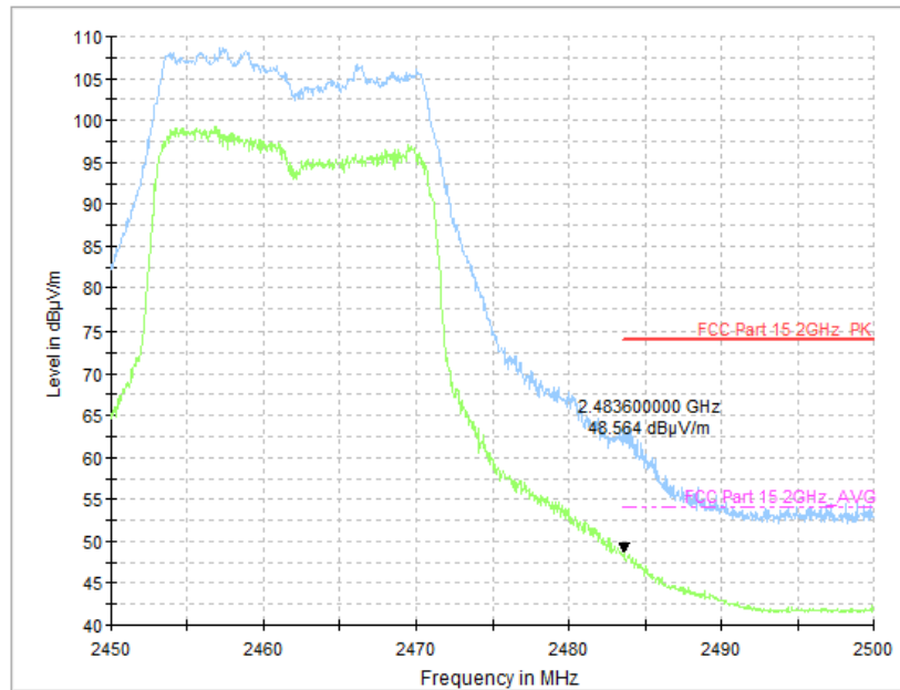
Fig.56 Radiated Restricted Band (802.11n HT20, CH11, 2.45GHz~2.5GHz, MIMO)
