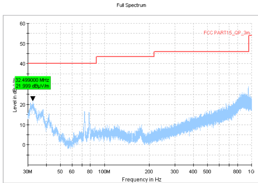
Fig.58 Radiated Spurious Emission (All Channels, 30MHz-1 GHz, MIMO)
