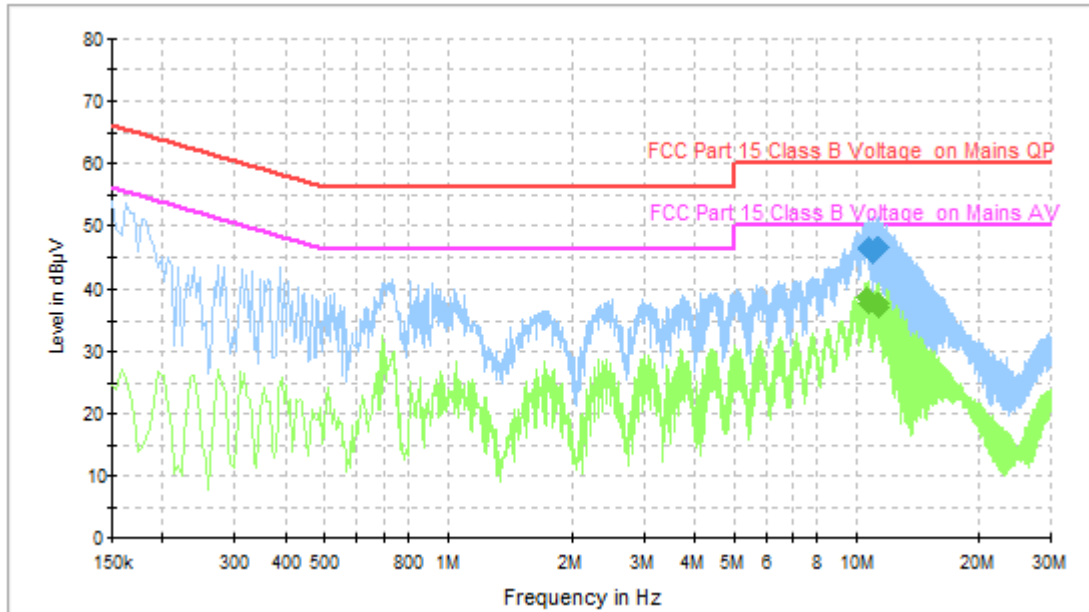
Fig.61 AC Power line Conducted Emission (Idle)
