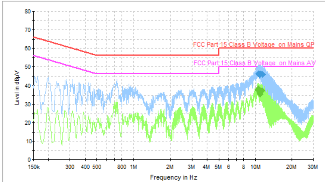
Fig.60 AC Power line Conducted Emission (Traffic)
