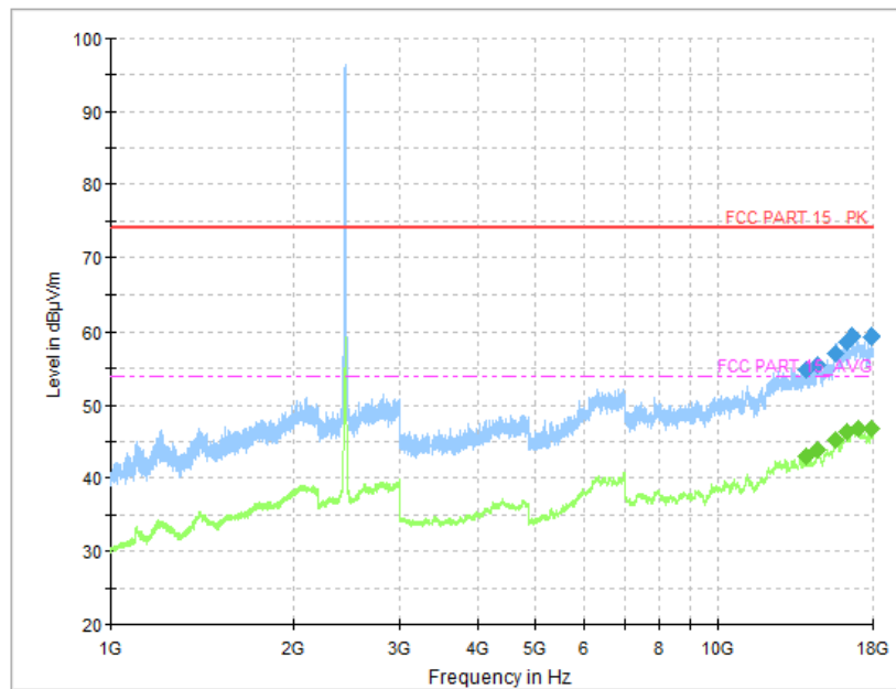
Fig.45 Radiated Spurious Emission (802.11n HT20, CH6, 1 GHz-18 GHz)
