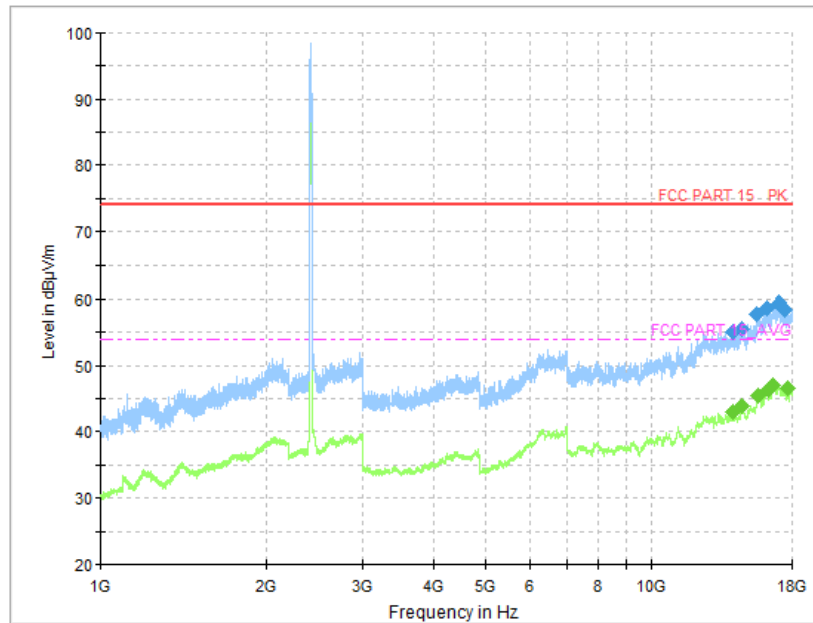
Fig.52 Radiated Spurious Emission (802.11n HT20, CH1, 1 GHz-18 GHz, MIMO)
