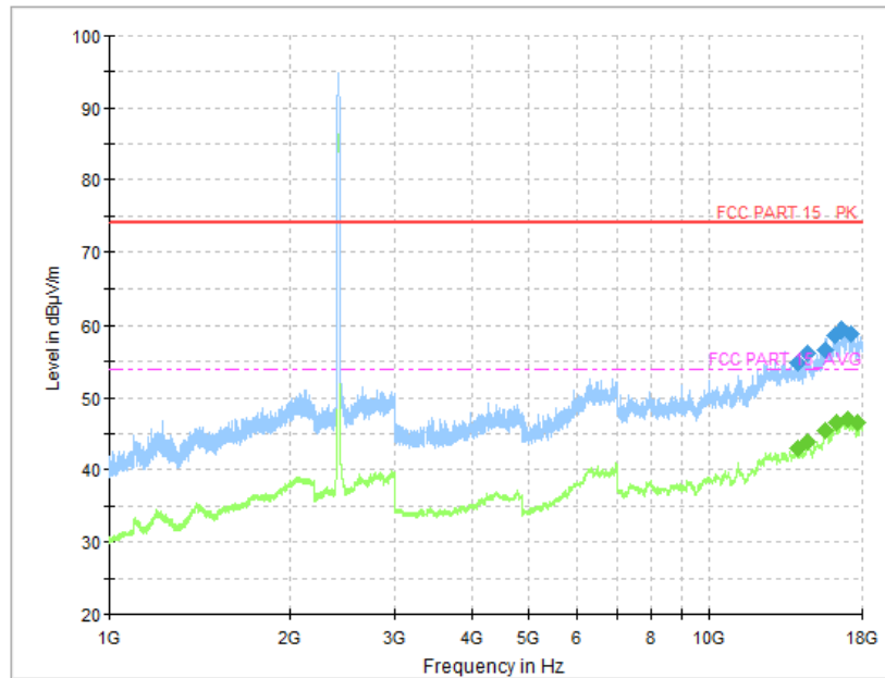
Fig.44 Radiated Spurious Emission (802.11n HT20, CH1, 1 GHz-18 GHz)
