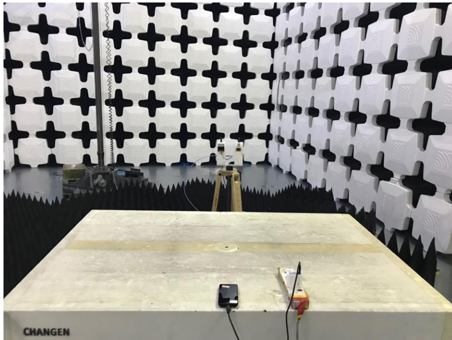
7. Radiated Emissions (Part 15B Camera/ Scanner/Video Player,18GHz-26.5GHz)
