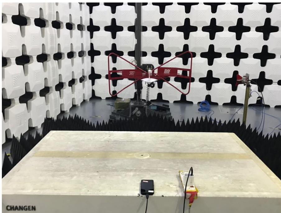
6. Radiated Emissions (Part 15B Camera/ Scanner/Video Player, 1GHz-18GHz)
