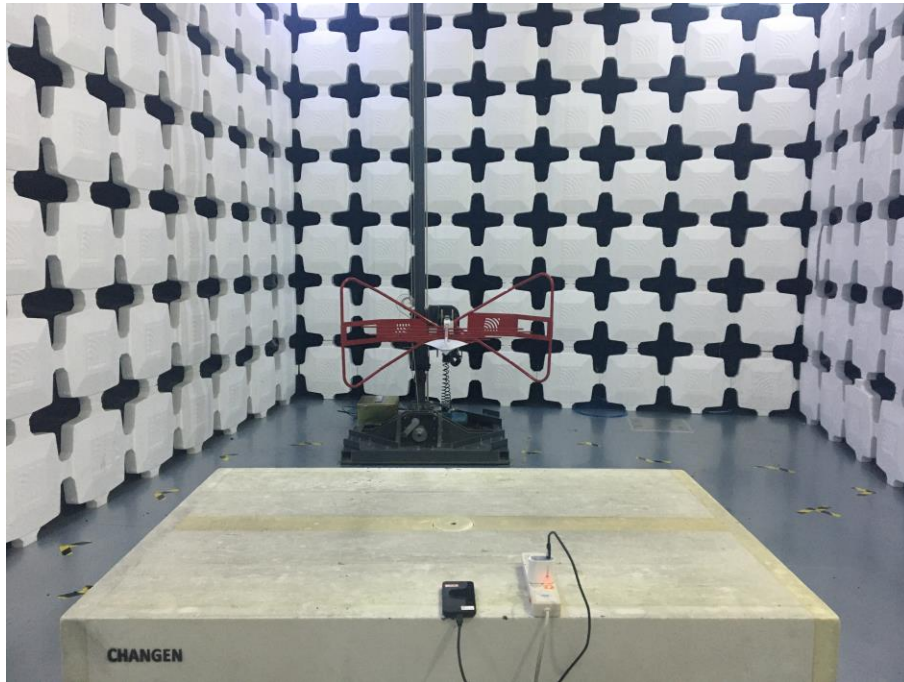
5. Radiated Emissions (Part 15B Camera/Scanner/Video Player, 30MHz-1GHz)
