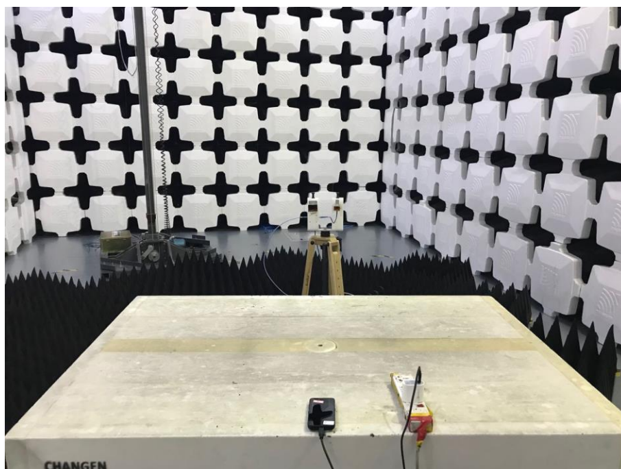
8. Radiated Emissions (Part 15B Camera/ Scanner/Video Player,26.5GHz-40GHz)
