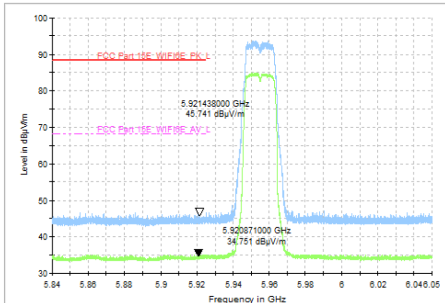
Fig. 1 Band Edges (802.11a, CH1 5955MHz)
