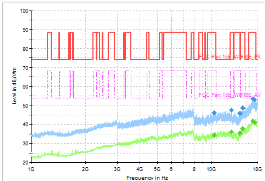
Fig. 11 Transmitter Spurious Emission (802.11a, CH1, 1GHz-18GHz)
