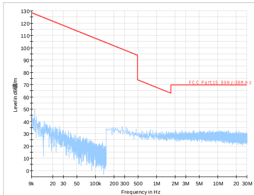
Fig. 60 Radiated Spurious Emission (All Channel, 9 kHz ~30 MHz)
