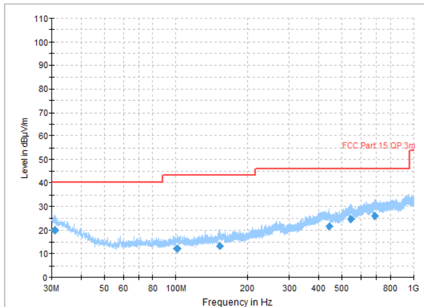
Fig. 57 Transmitter Spurious Emission (All channel, 30MHz~1GHz)
