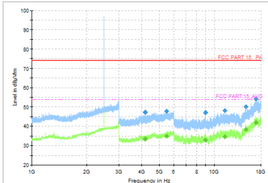
Fig. 13 Radiated Spurious Emission (8DPSK, CH78, 1GHz ~18GHz)
