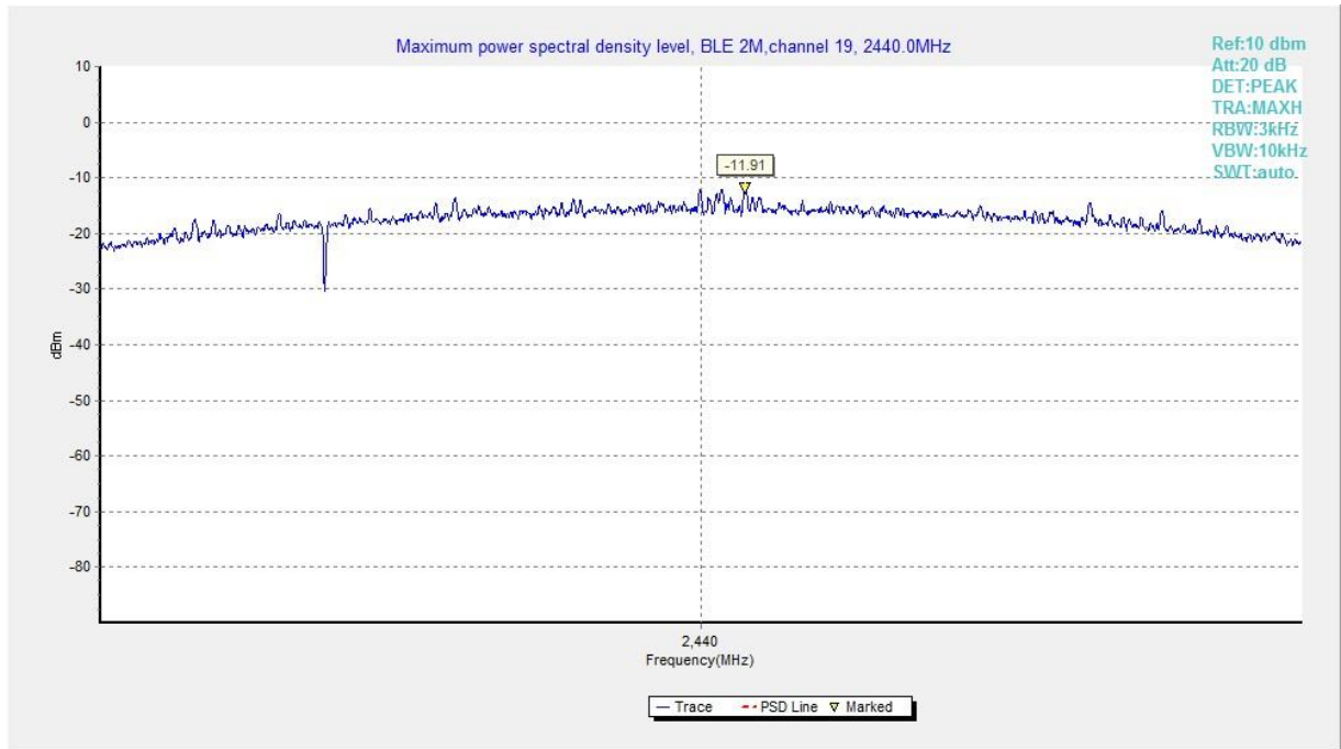
Fig.2 Power Spectral Density (Ch 19), LE 2M
