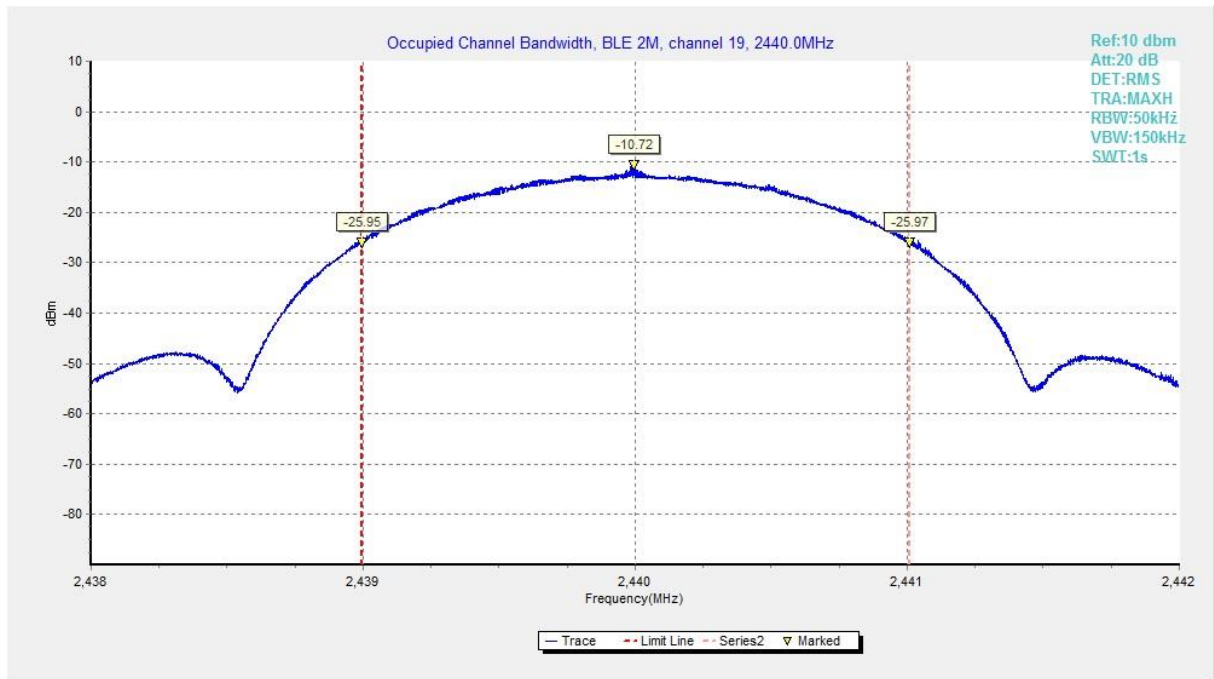
Fig.2 99% Occupied Bandwidth (Ch 19), LE 2M
