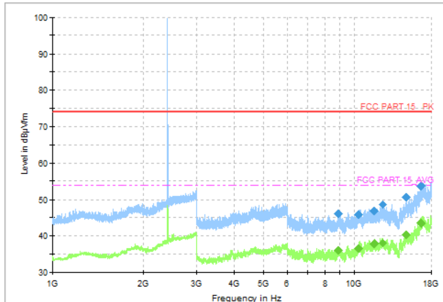
Fig.1 Radiated Spurious Emission (Ch0, 1 GHz - 18 GHz), 1M
