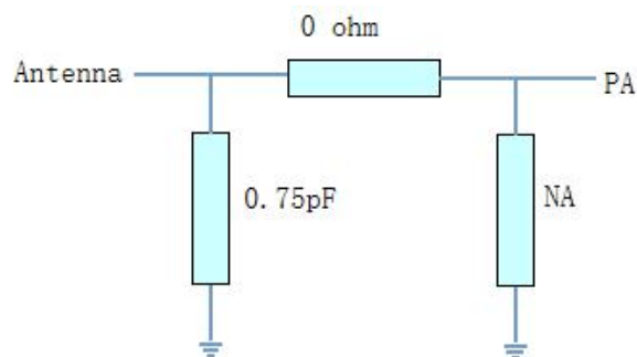
Picture 5 Matching network of WIFI-ANT1 antenna
