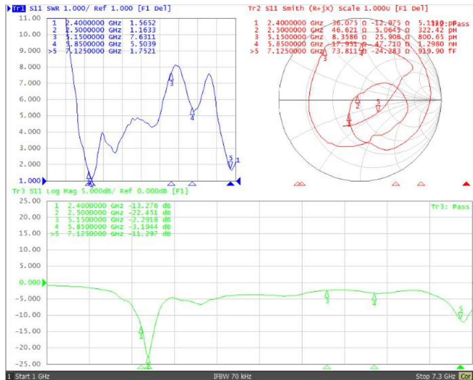
Picture 8 Return Loss of WIFI-ANT0 antenna
