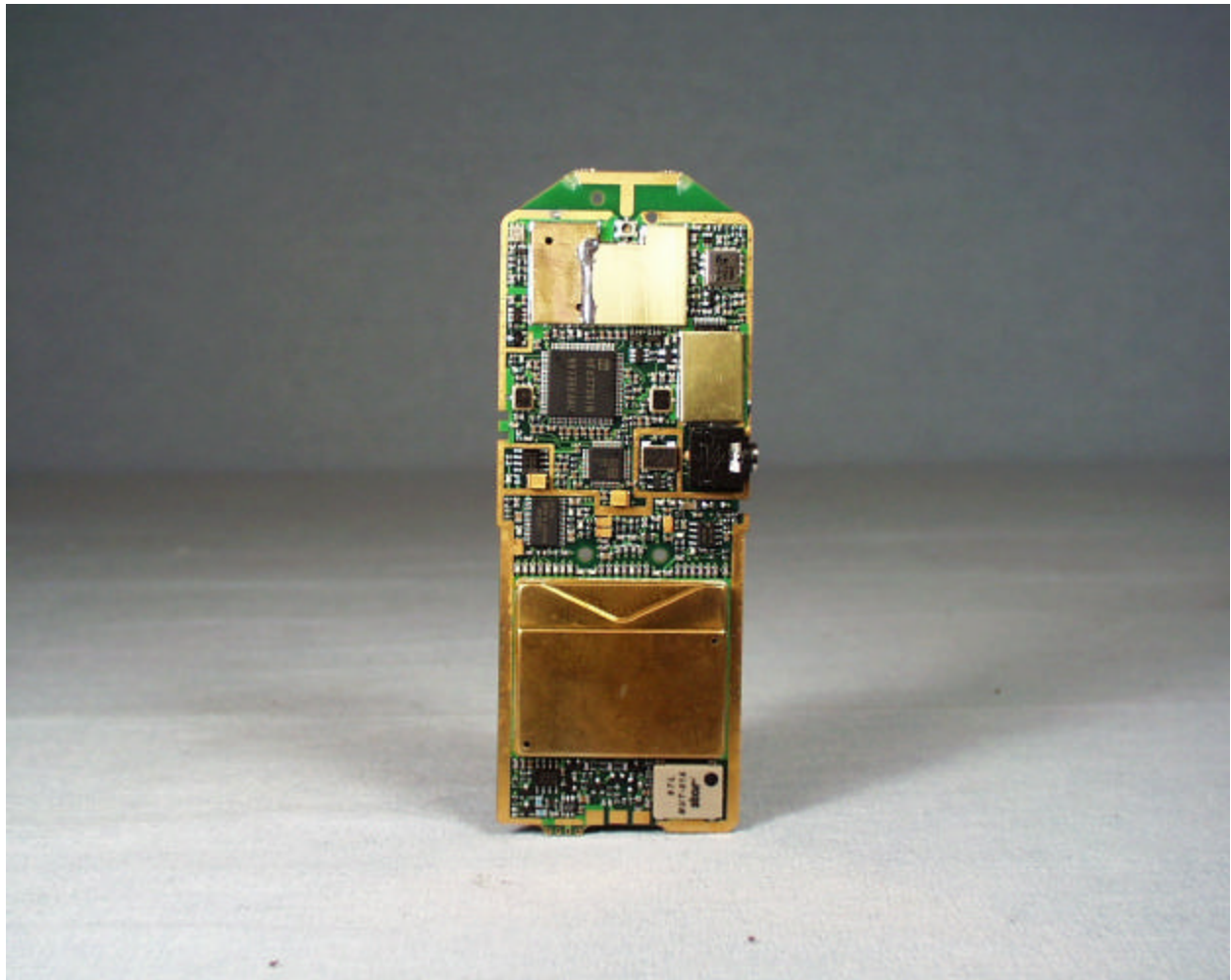
Inside View - Side B with RF cans installed
