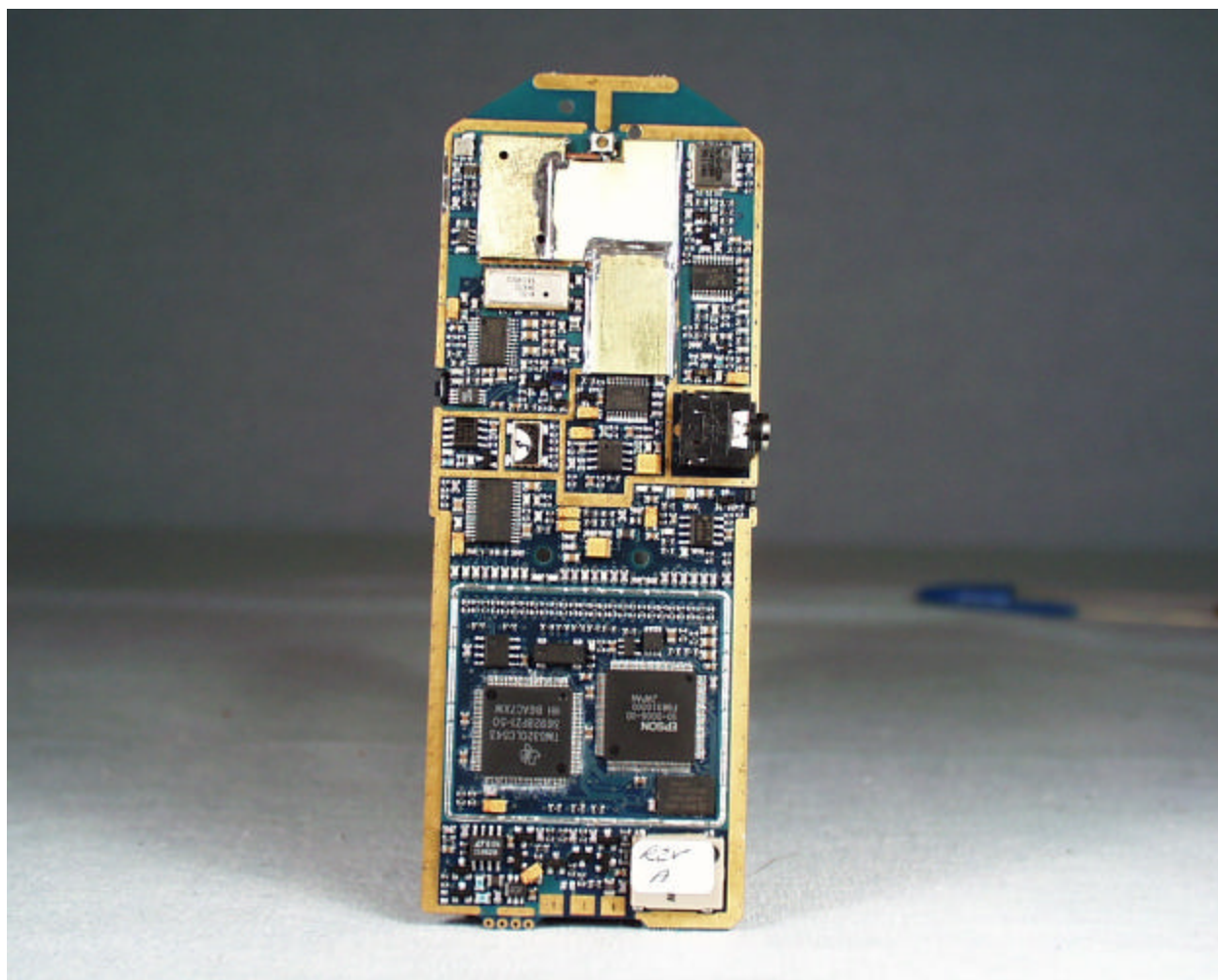
Inside View - Side B with RF cans installed
