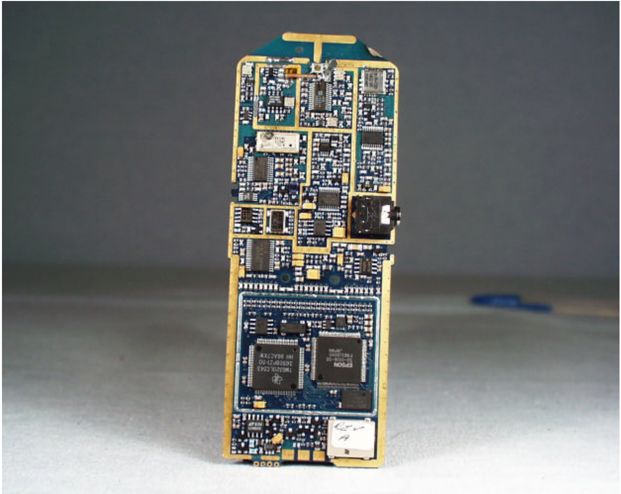
Inside View - Side B with RF cans removed
