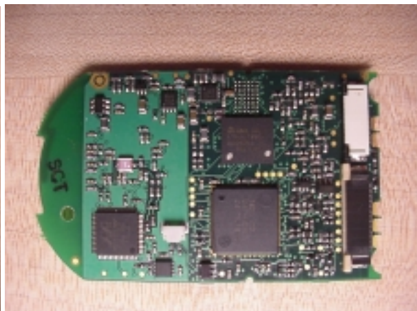
SNP2400 RF Generation Board – Side B
