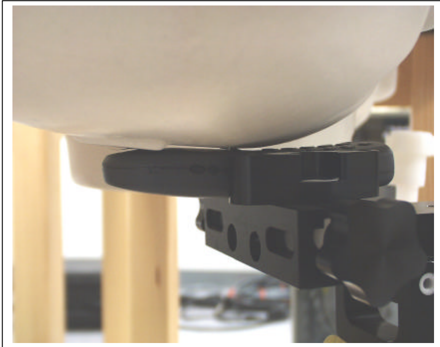
EUT Setup Configuration 2 (Right Head - Touched position)
