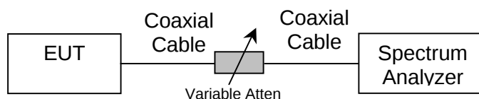
Measurement setup for 6dB bandwidth test
