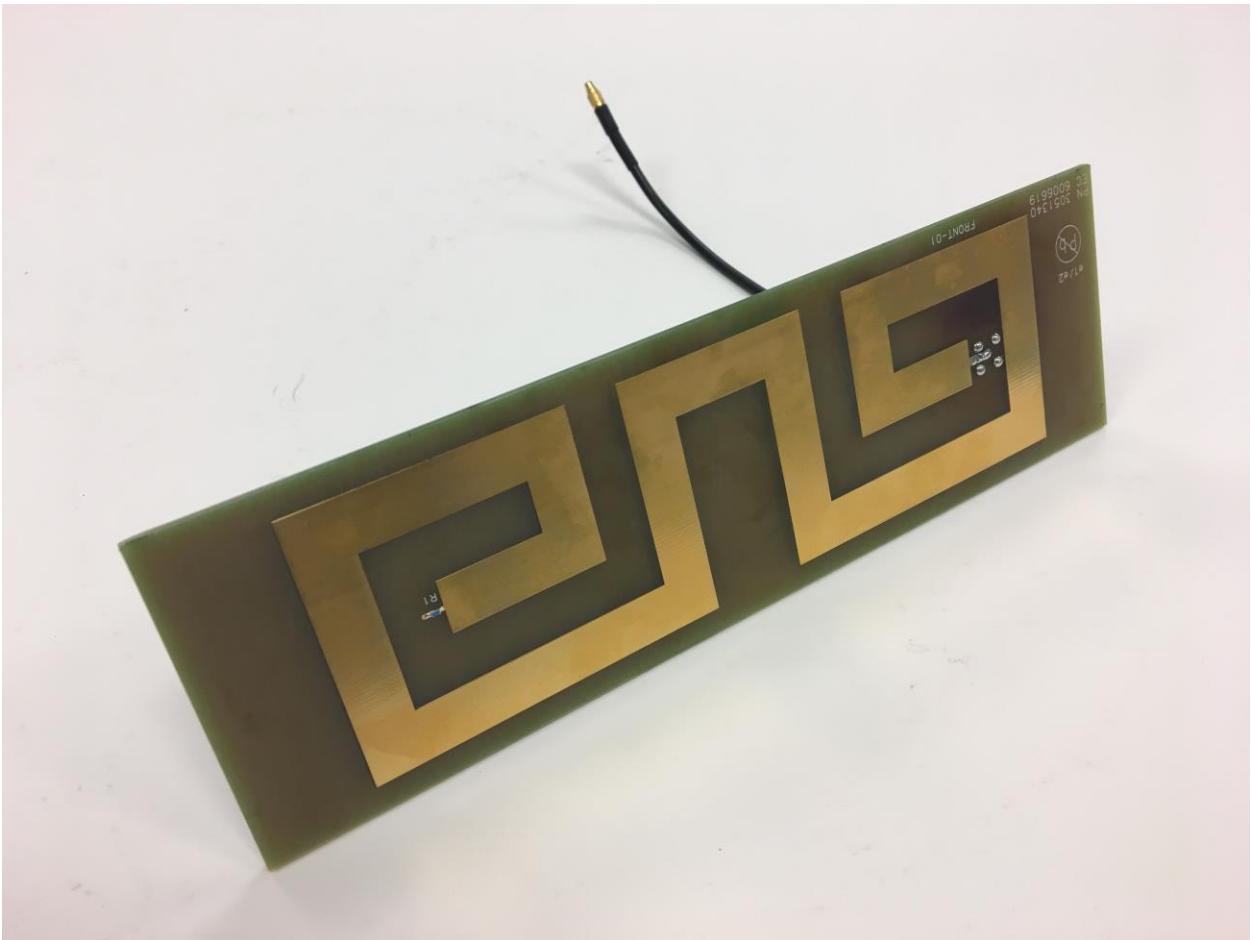
Front view of antenna.
