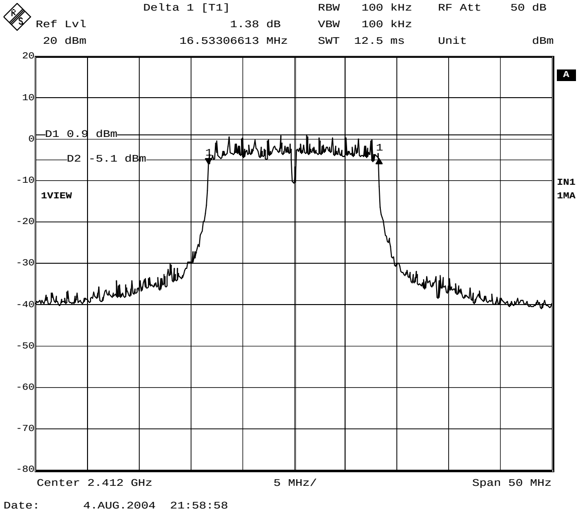
Figure 12: 6 dB Bandwidth – Channel 1, 64QAM, 54 Mbps
