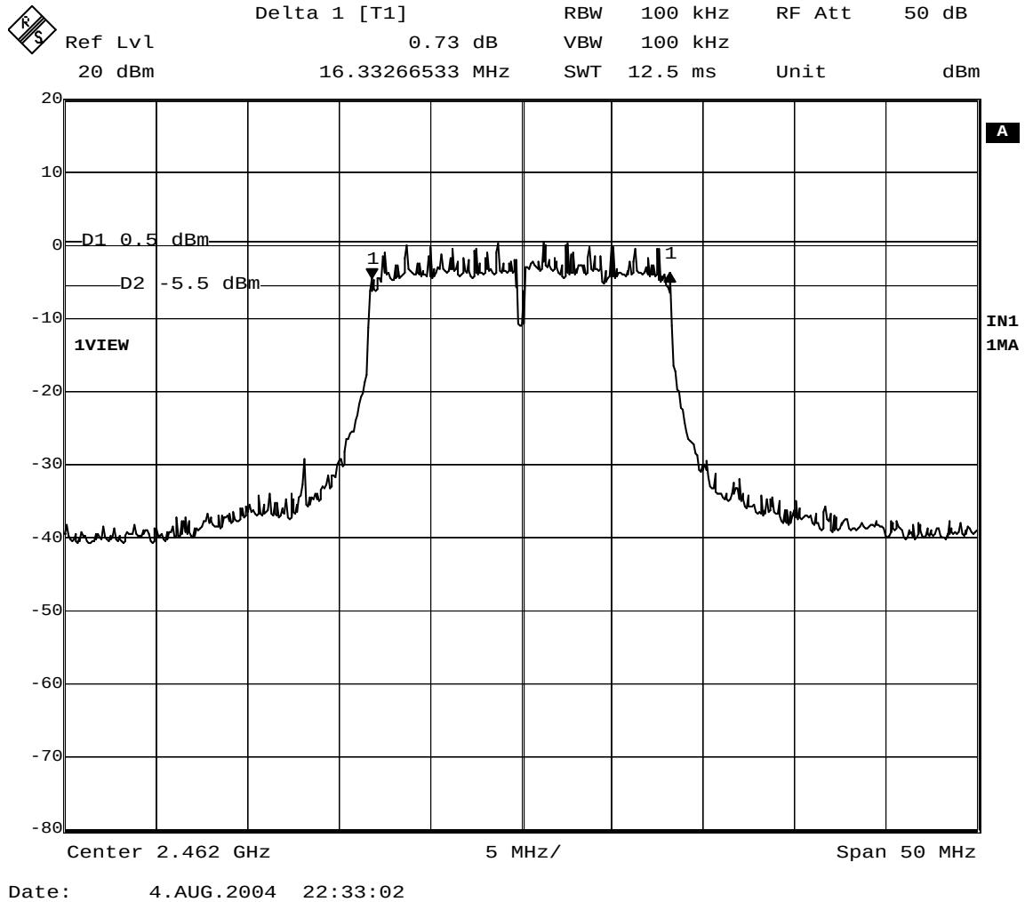
Figure 18: 6 dB Bandwidth – Channel 11, 64QAM, 54 Mbps
