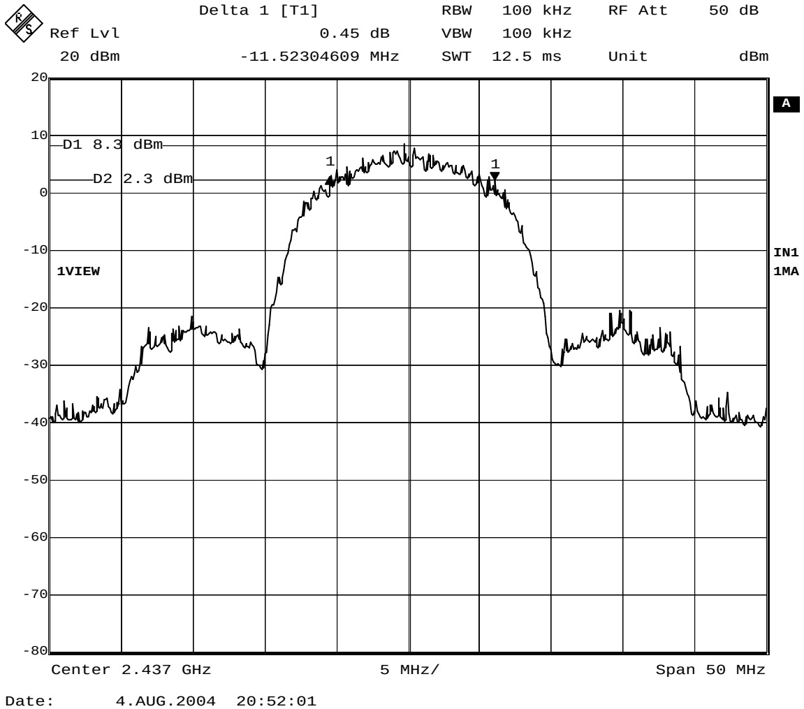
Figure 2: 6 dB Bandwidth – Channel 6, CCK, 11 Mbps
