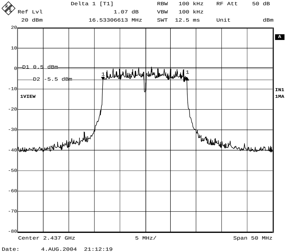
Figure 6: 6 dB Bandwidth – Channel 6, 64QAM, 54 Mbps
