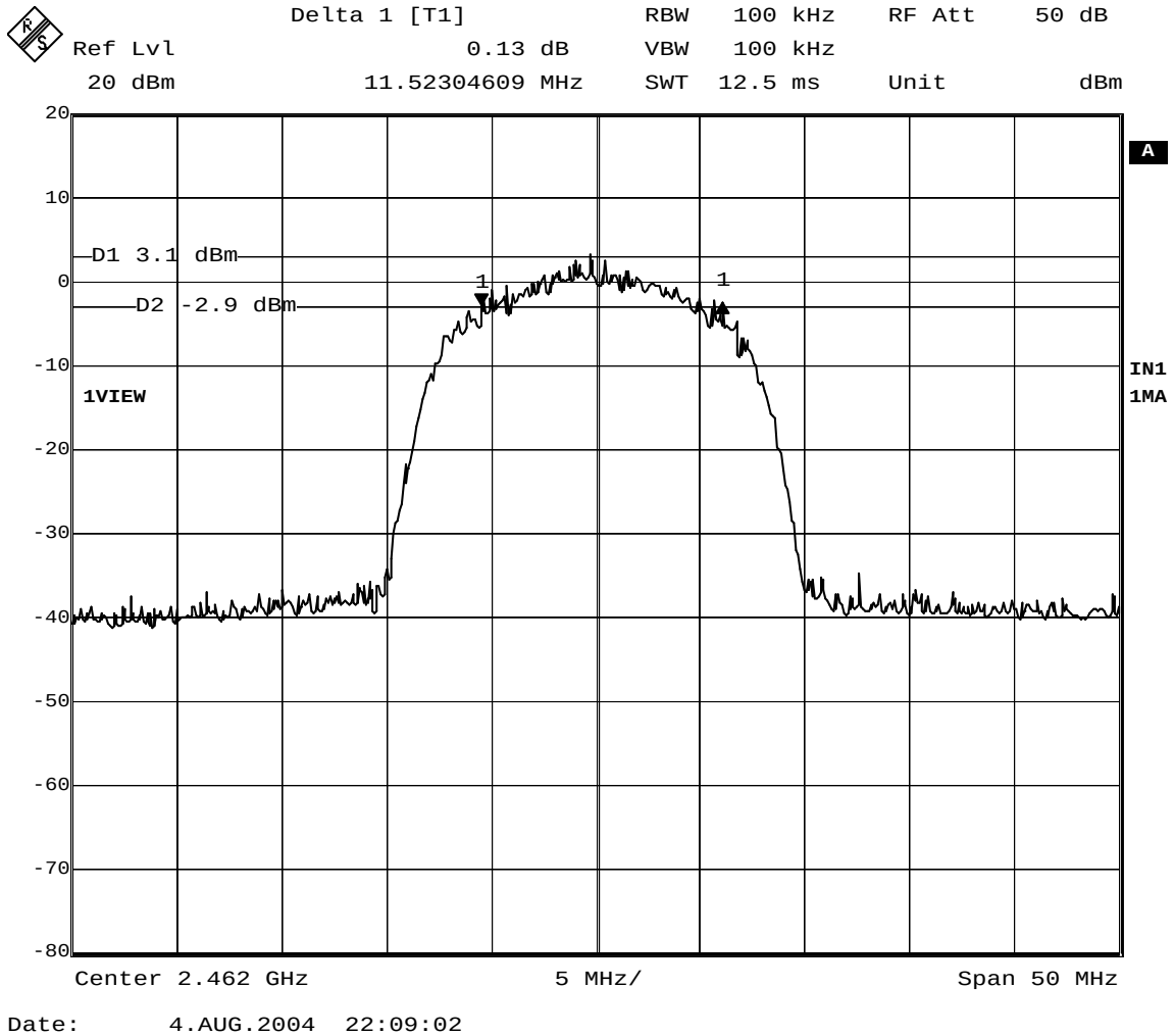
Figure 14: 6 dB Bandwidth – Channel 11, CCK, 11 Mbps
