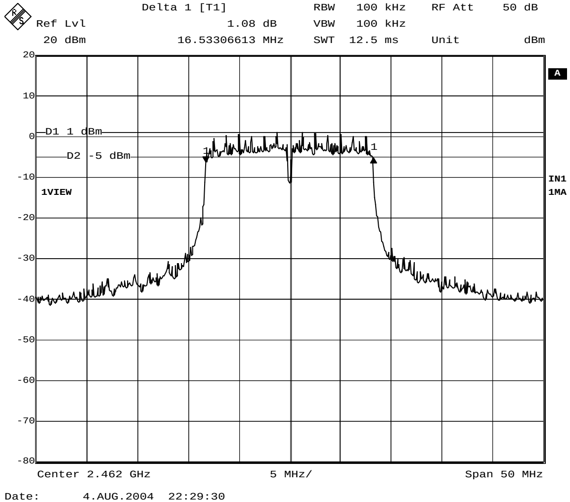
Figure 17: 6 dB Bandwidth – Channel 11, 16QAM, 36 Mbps
