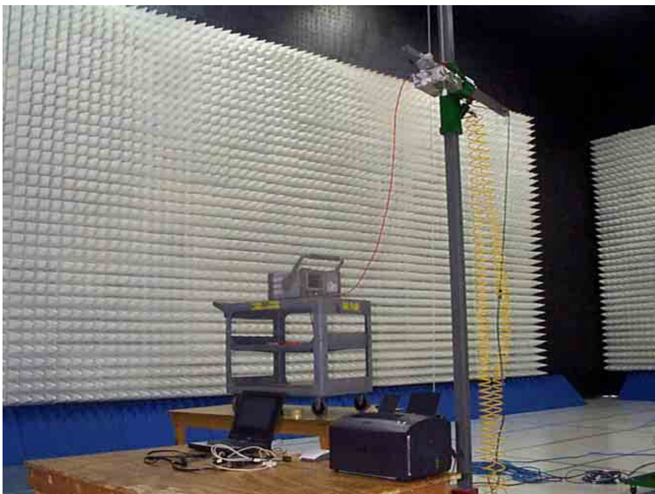
Figure 3: Radiated Testing to 26GHz
