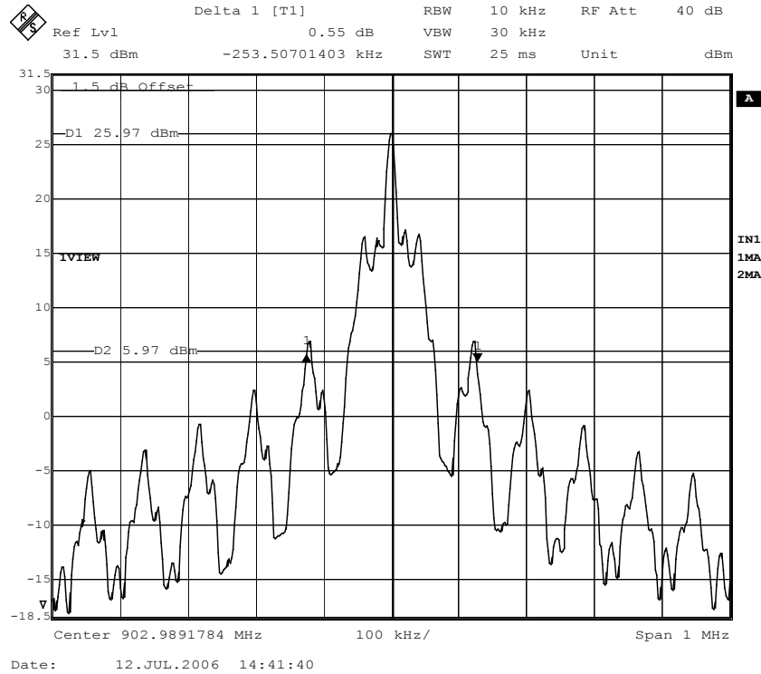
Figure 16. 20 dB Bandwidth, ISO 18000-6B, Channel 1.
