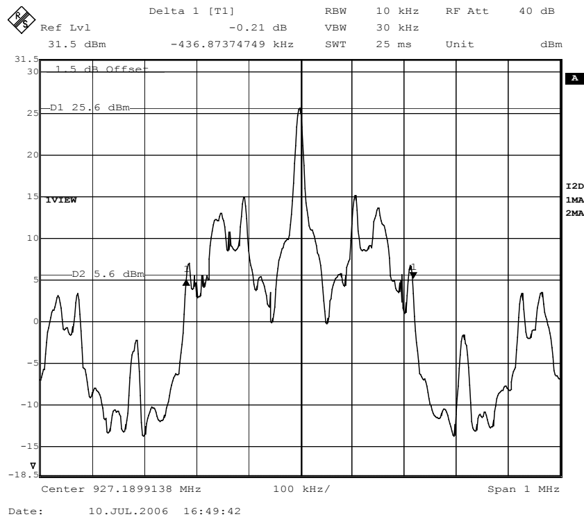
Figure 15. 20 dB Bandwidth, EPC Gen2, Channel 53.
