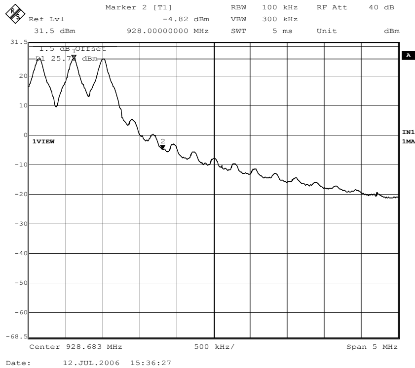
Figure 47. Band edge compliance; EPC Class 0 mode; Channel 53, hopping enabled.
