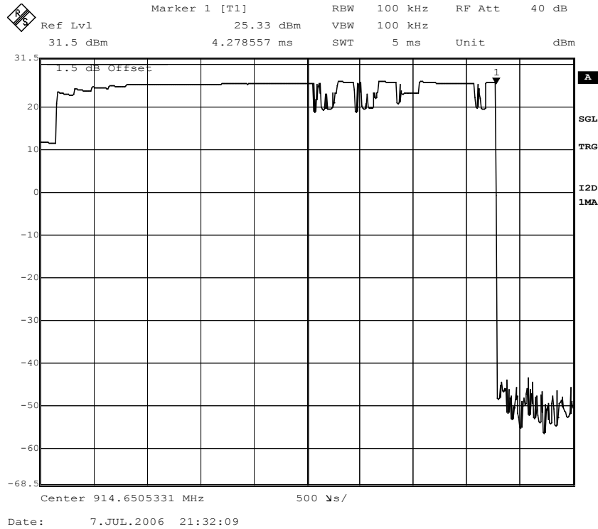
Figure 24. ON time; Channel 26.
