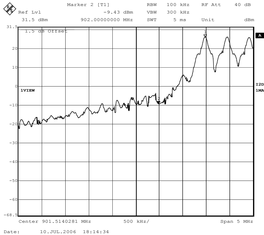
Figure 41. Band edge compliance; EPC Gen2 mode; Channel 1, hopping enabled.
