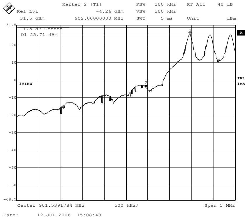
Figure 49. Band edge compliance; EPC Class 1 mode; Channel 1, hopping enabled.
