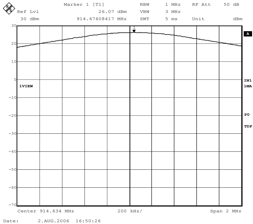
Figure 34. Conducted output power; Channel 26, 115% nominal voltage.
