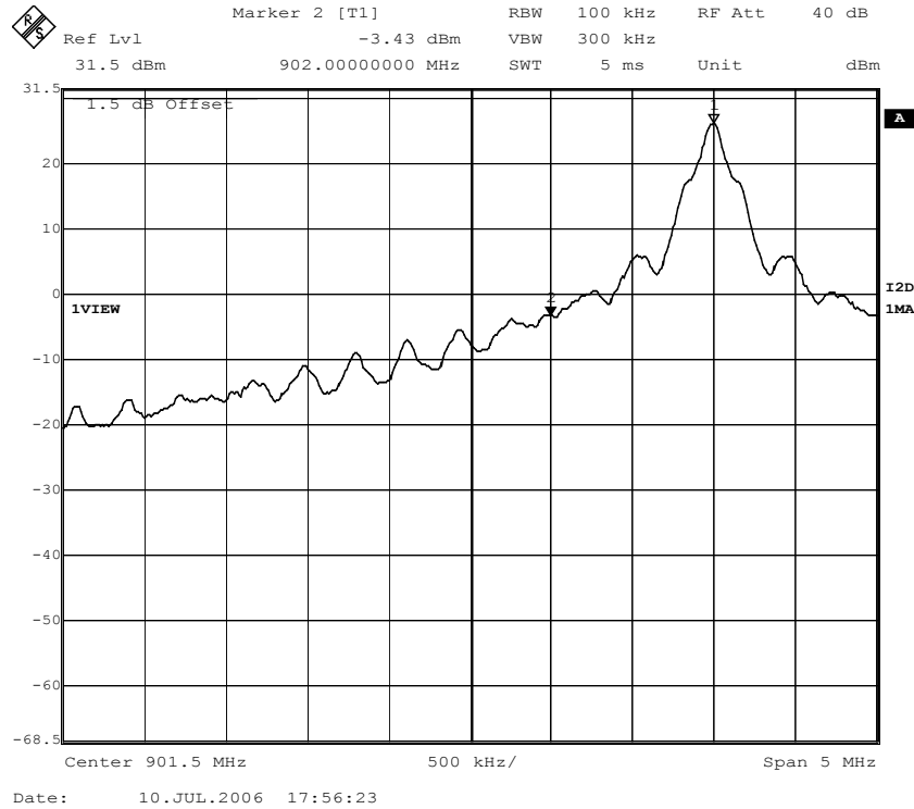
Figure 40. Band edge compliance; EPC Gen2 mode; Channel 1, hopping disabled.
