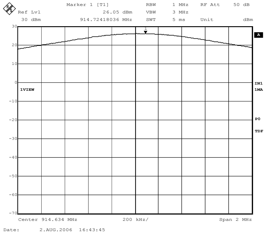
Figure 31. Conducted output power; Channel 26, 85% nominal voltage.
