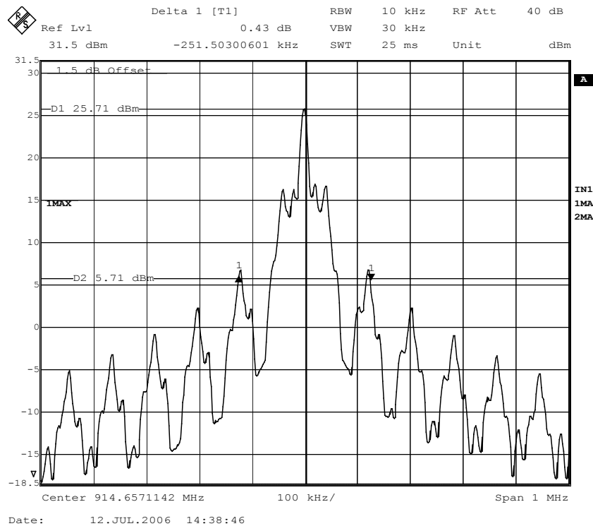
Figure 17. 20 dB Bandwidth, ISO 18000-6B, Channel 26.
