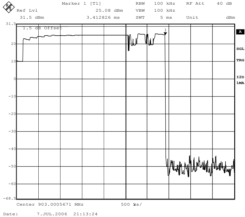
Figure 22. ON time; Channel 1.
