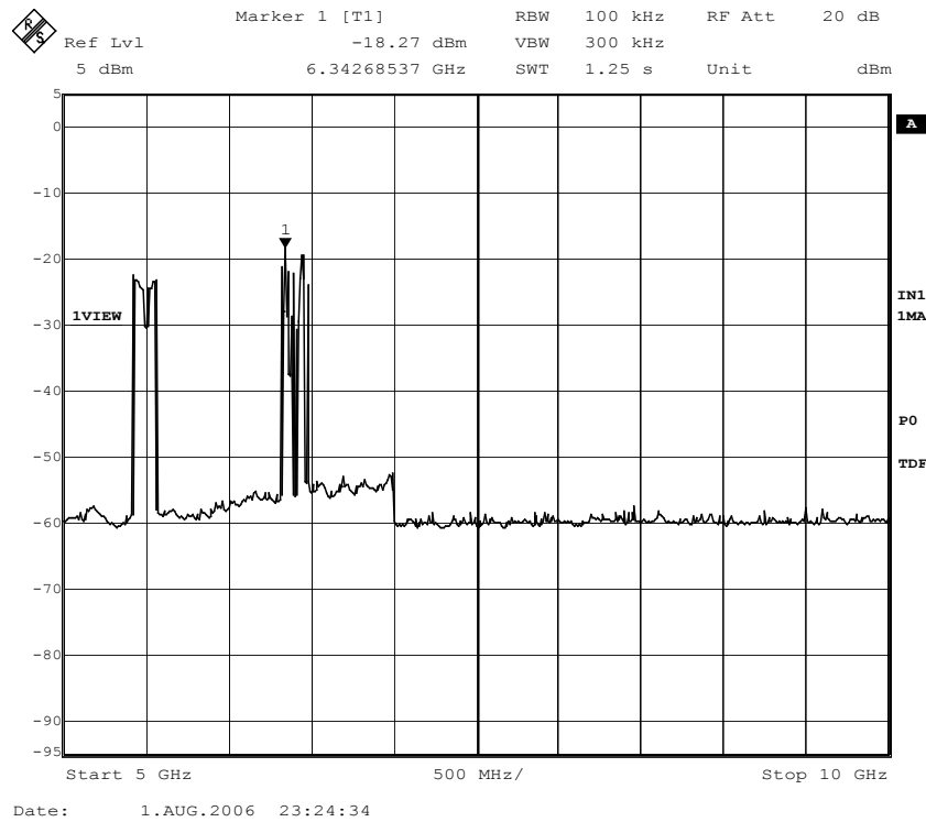
Figure 39. Out of band emissions at antenna port; 5 GHz - 10 GHz.
