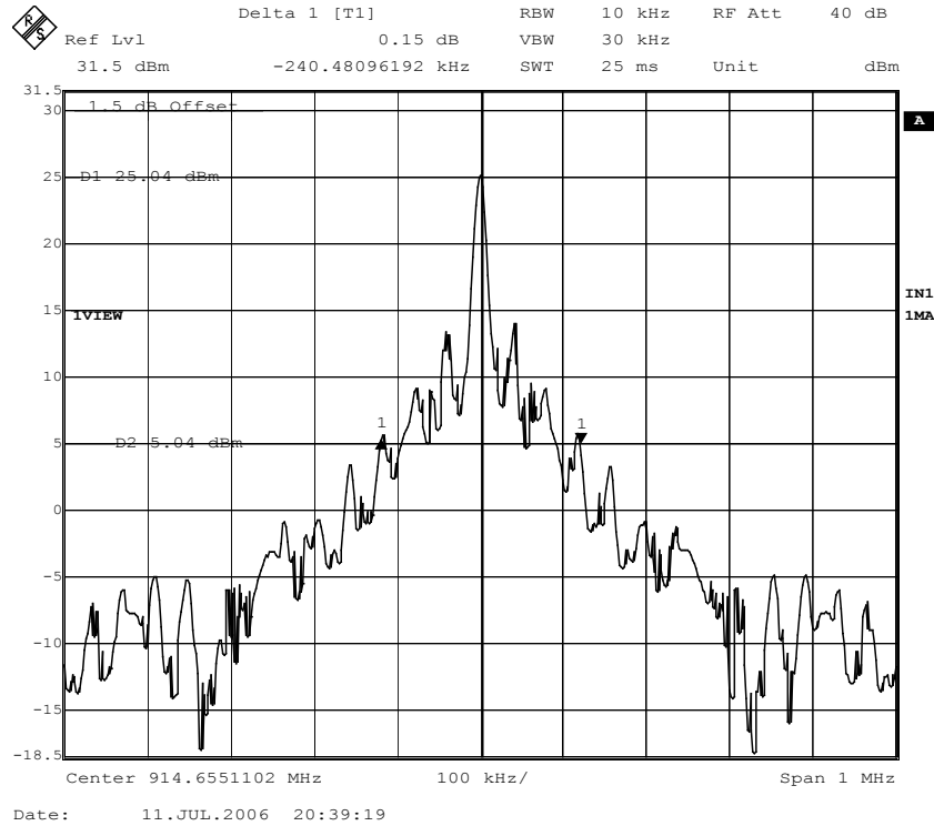
Figure 8. 20 dB Bandwidth, EPC Class 0, Channel 26.
