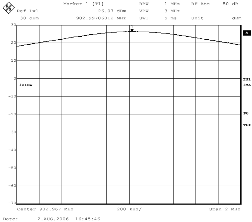
Figure 30. Conducted output power; Channel 1, 85% nominal voltage.
