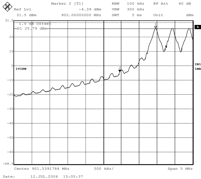
Figure 45. Band edge compliance; EPC Class 0 mode; Channel 1, hopping enabled.
