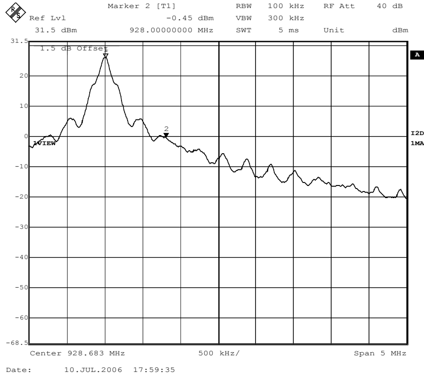
Figure 42. Band edge compliance; EPC Gen2 mode; Channel 53, hopping disabled.
