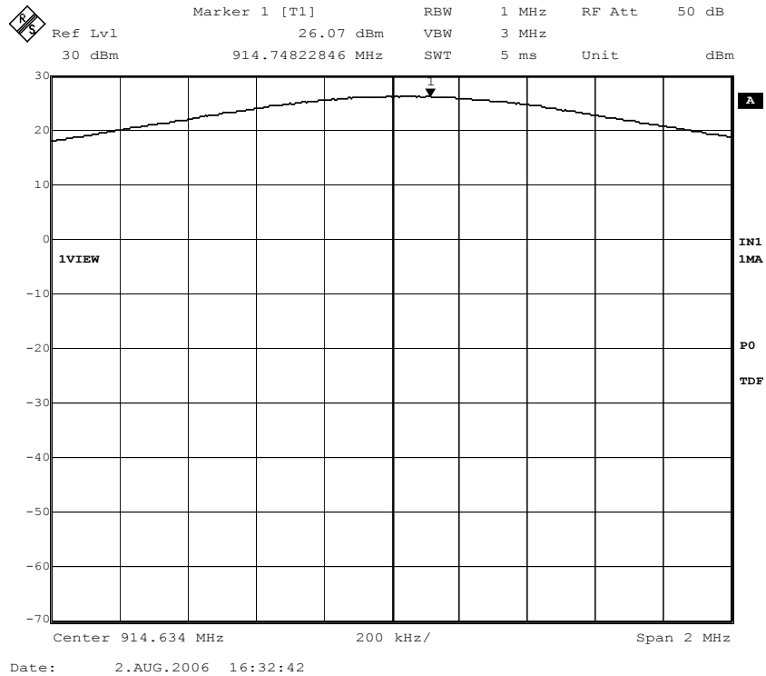
Figure 28. Conducted output power; Channel 26, nominal voltage.
