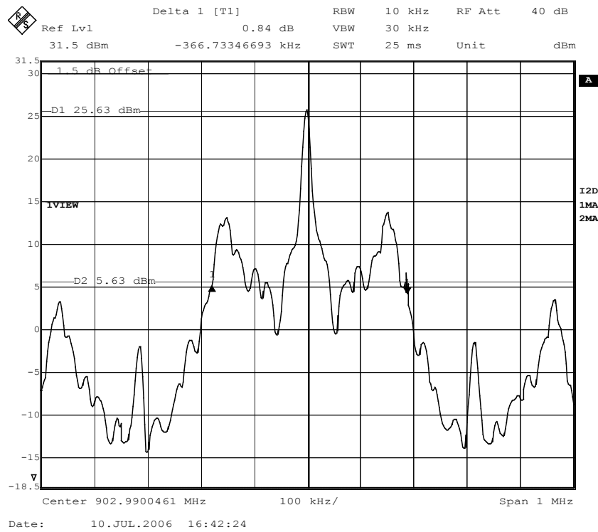
Figure 13. 20 dB Bandwidth, EPC Gen2, Channel 1.
