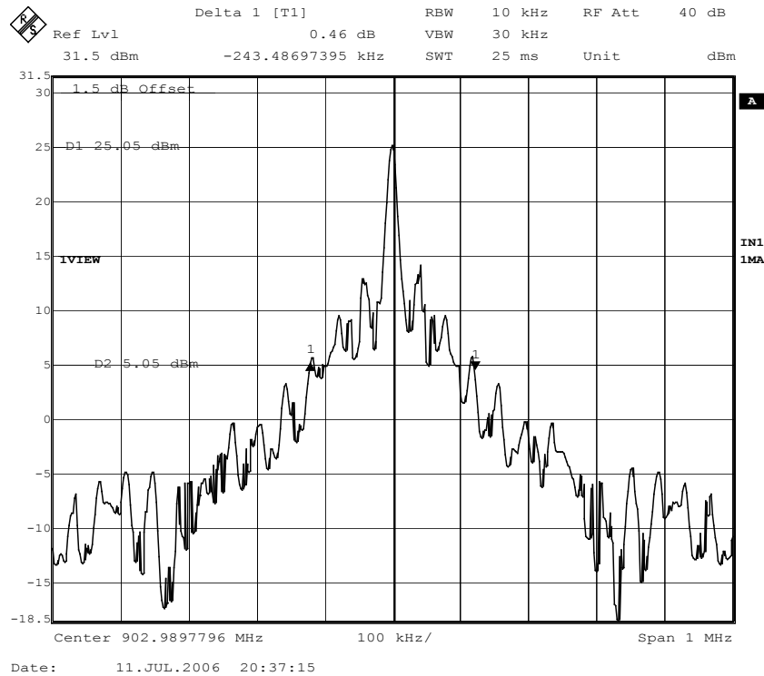
Figure 7. 20 dB Bandwidth, EPC Class 0, Channel 1.
