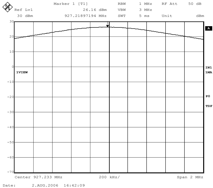
Figure 32. Conducted output power; Channel 53, 85% nominal voltage.
