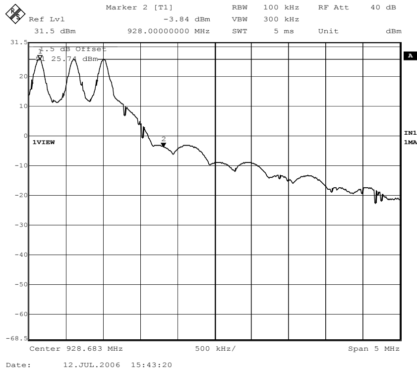
Figure 51. Band edge compliance; EPC Class 1 mode; Channel 53, hopping enabled.
