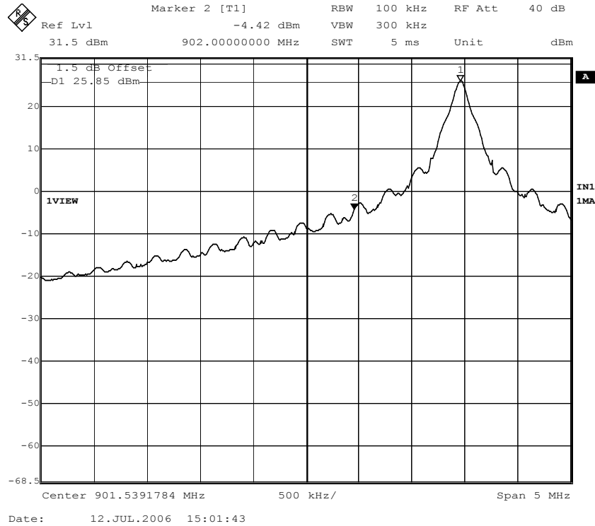
Figure 44. Band edge compliance; EPC Class 0 mode; Channel 1, hopping disabled.
