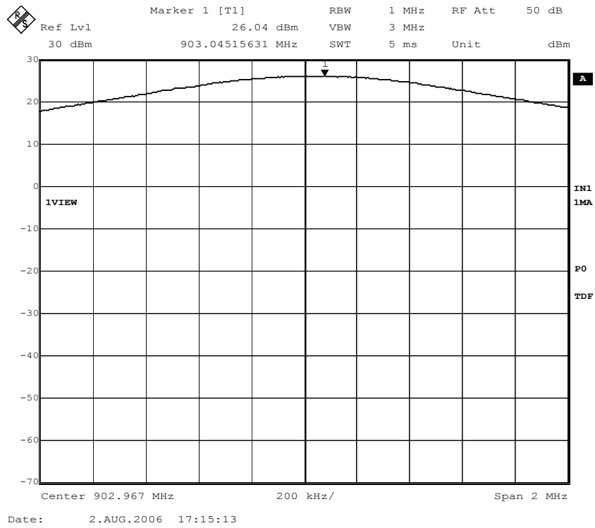
Figure 33. Conducted output power; Channel 1, 115% nominal voltage.
