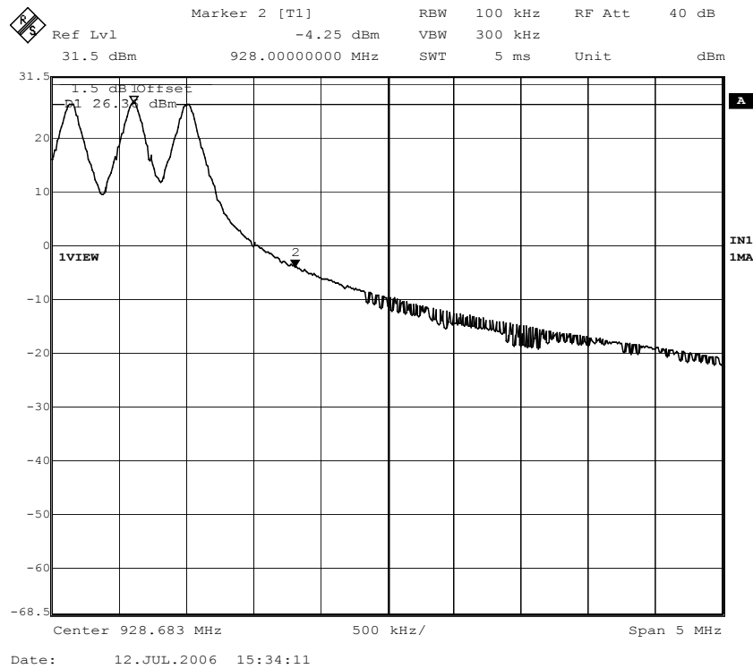
Figure 55. Band edge compliance; ISO 18000-6B mode; Channel 53, hopping enabled.
