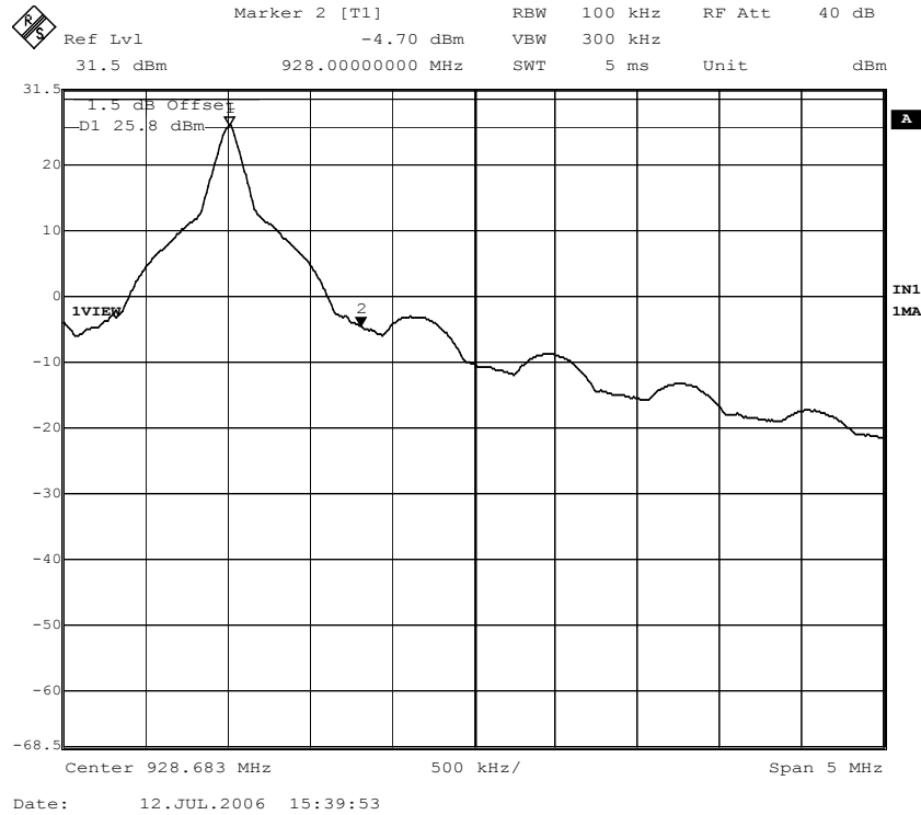
Figure 50. Band edge compliance; EPC Class 1 mode; Channel 53, hopping disabled.
