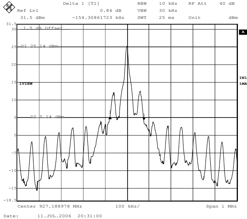
Figure 12. 20 dB Bandwidth, EPC Class 1, Channel 53.
