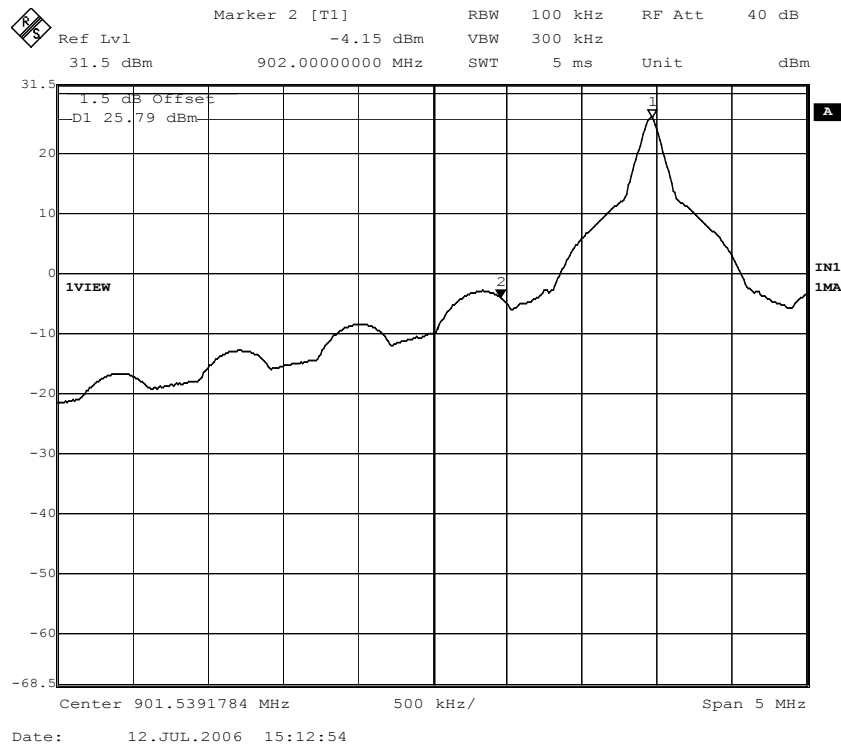
Figure 48. Band edge compliance; EPC Class 1 mode; Channel 1, hopping disabled.
