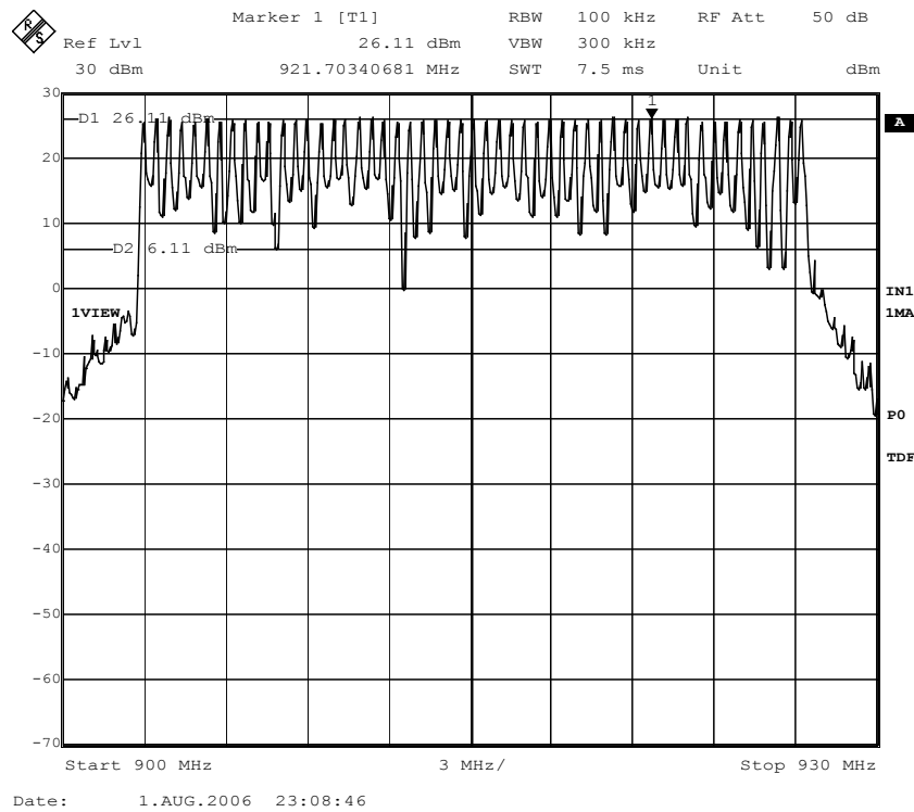
Figure 36. In band emissions at antenna port; 900 MHz - 930 MHz.
