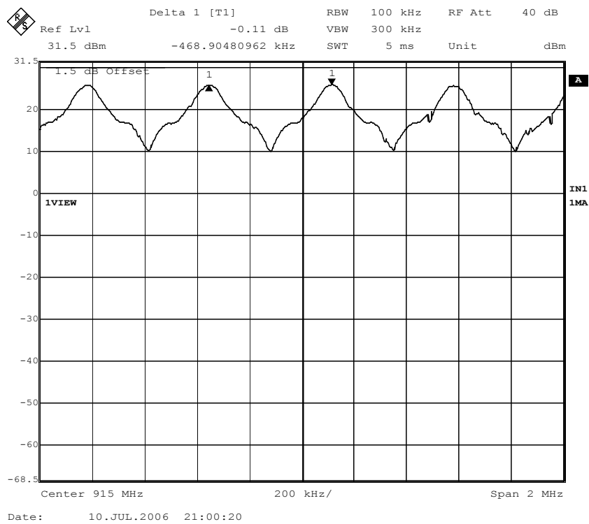
Figure 19. Hopping channel separation.
