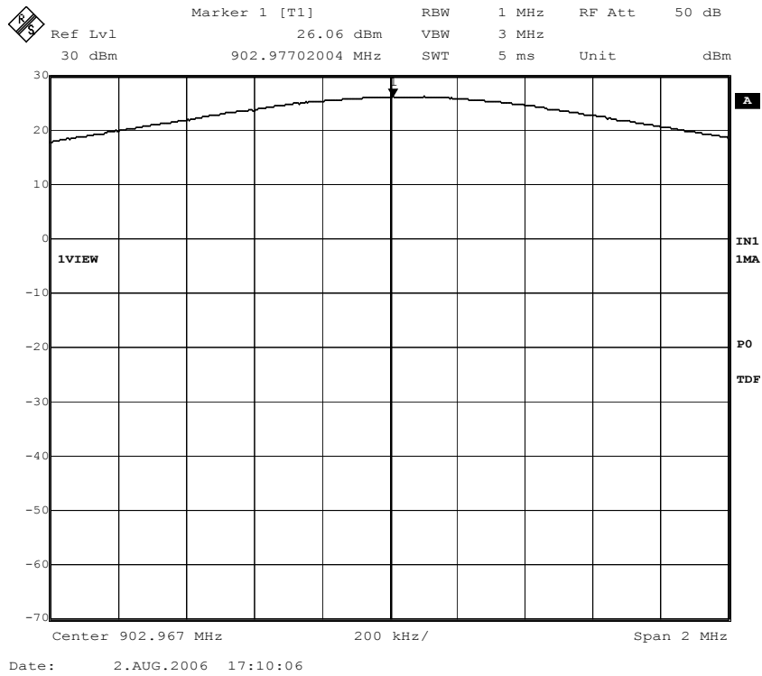
Figure 27. Conducted output power; Channel 1, nominal voltage.
