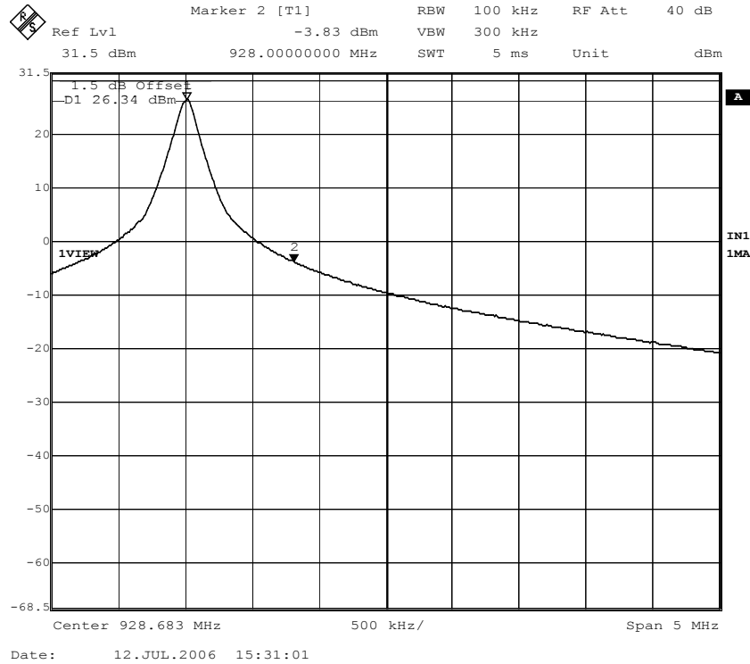
Figure 54. Band edge compliance; ISO 18000-6B mode; Channel 53, hopping disabled.
