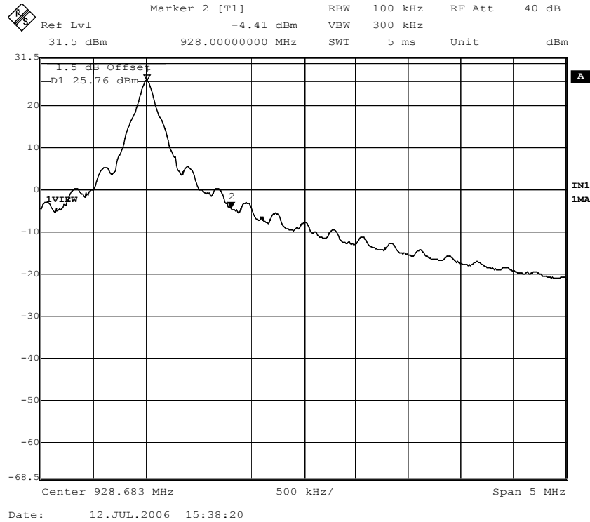
Figure 46. Band edge compliance; EPC Class 0 mode; Channel 53, hopping disabled.
