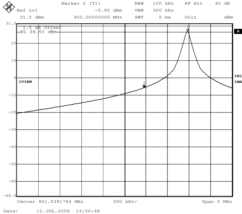
Figure 52. Band edge compliance; ISO 18000-6B mode; Channel 1, hopping disabled.
