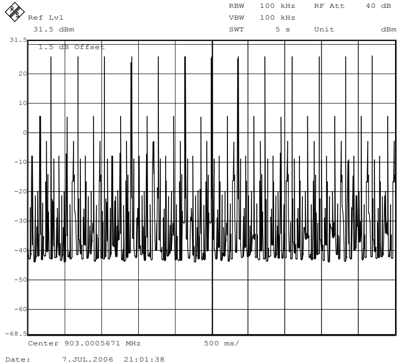
Figure 21. Number of ON events in a 5 second sweep; Channel 1.
