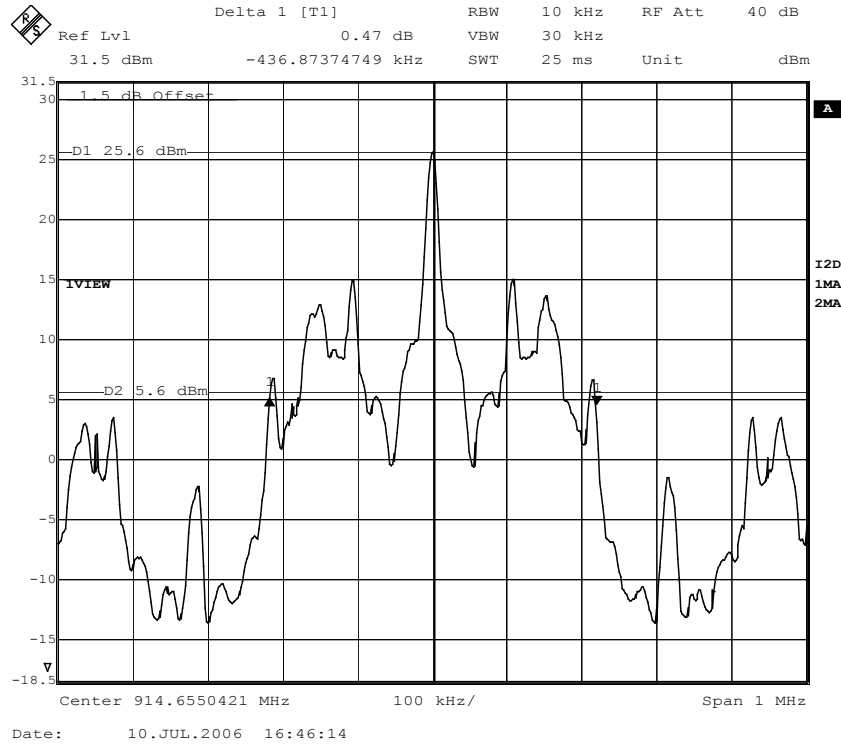
Figure 14. 20 dB Bandwidth, EPC Gen2, Channel 26.
