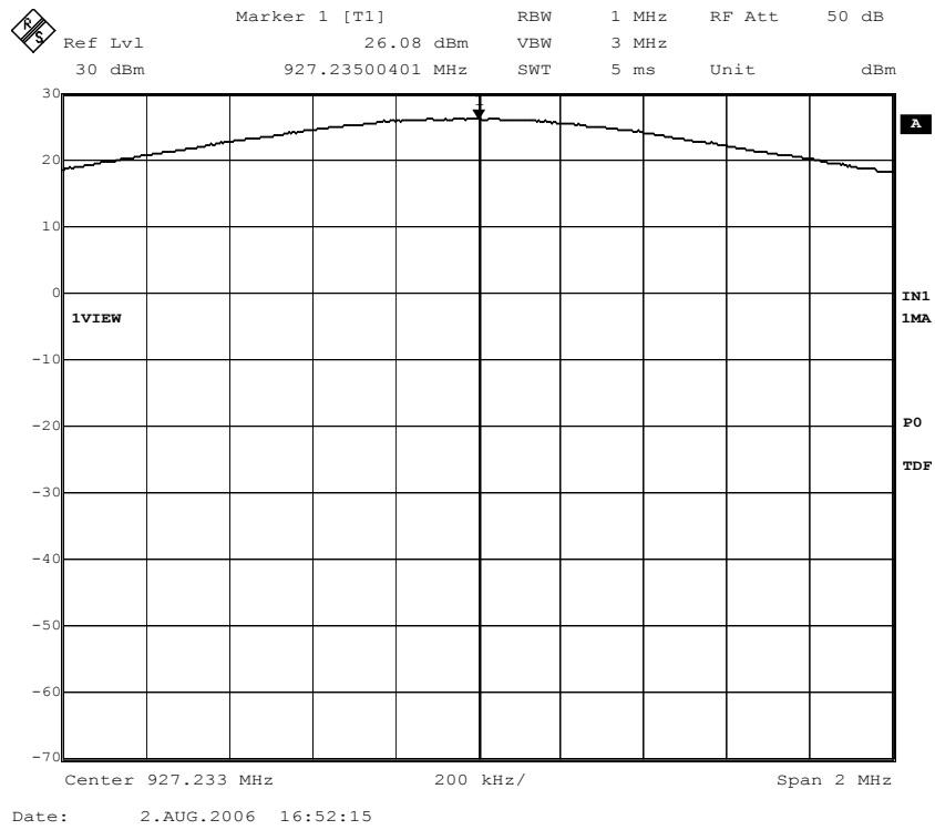
Figure 35. Conducted output power; Channel 53, 115% nominal voltage.
