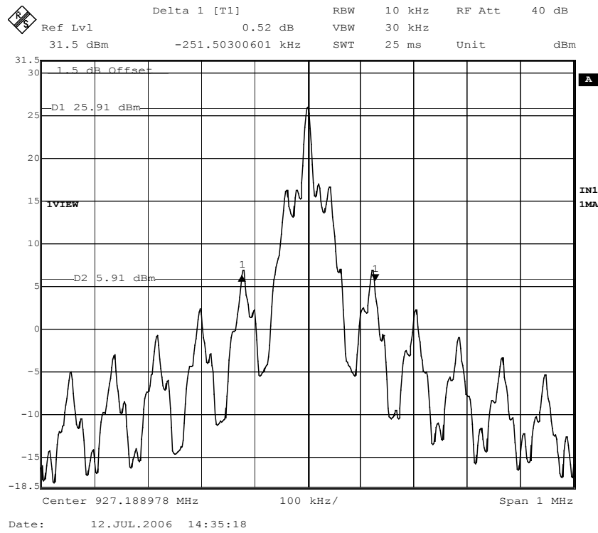
Figure 18. 20 dB Bandwidth, ISO 18000-6B, Channel 53.
