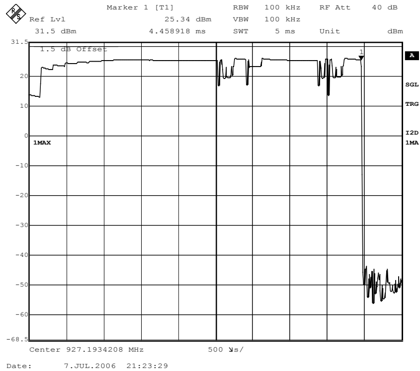
Figure 26. ON time; Channel 53.
