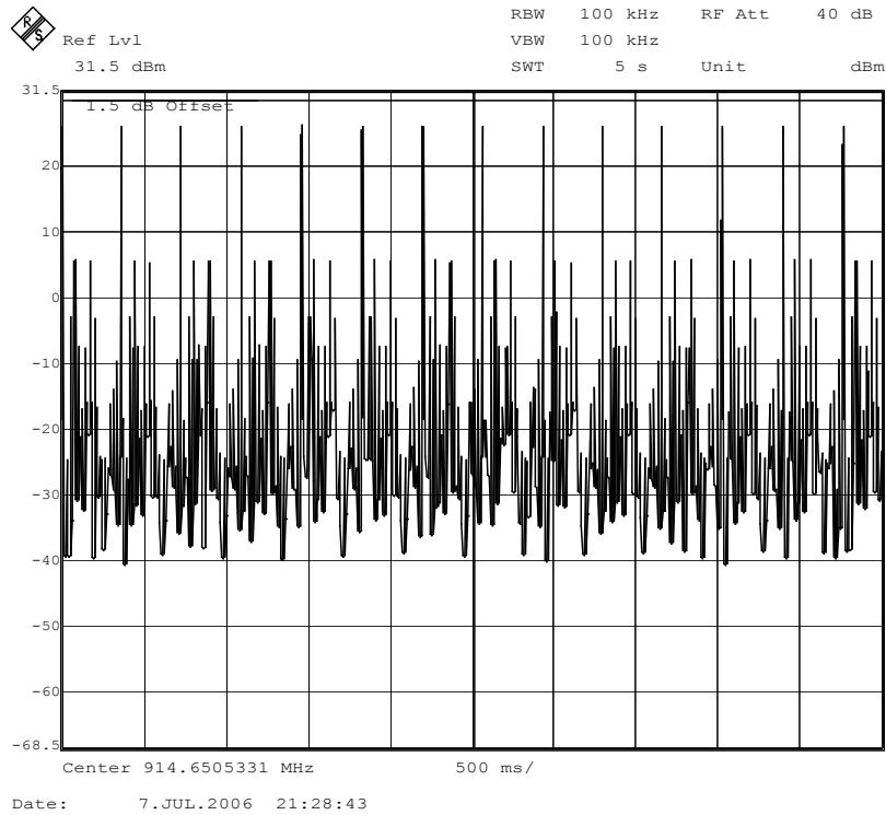
Figure 23. Number of ON events in a 5 second sweep; Channel 26.
