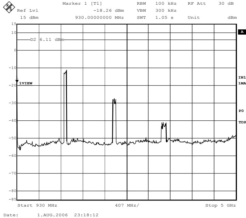
Figure 38. Out of band emissions at antenna port; 930 MHz - 5 GHz.
