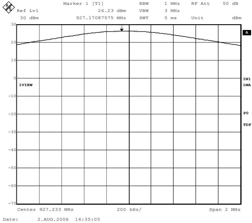
Figure 29. Conducted output power; Channel 53, nominal voltage.
