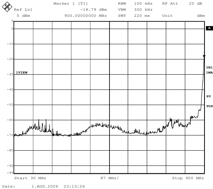
Figure 37. Out of band emissions at antenna port; 30 MHz - 900 MHz.
