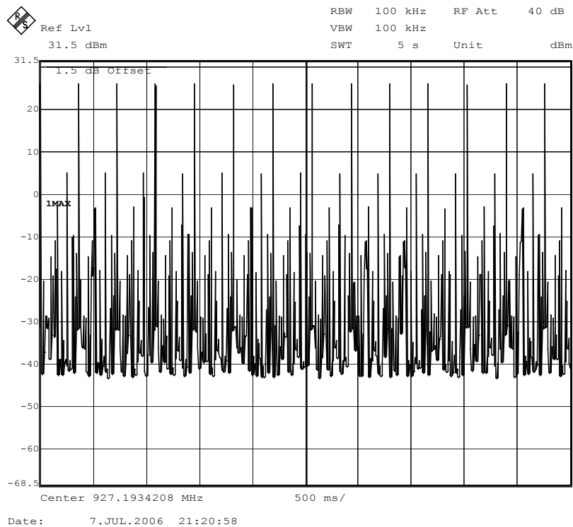
Figure 25. Number of ON events in a 5 second sweep; Channel 53.
