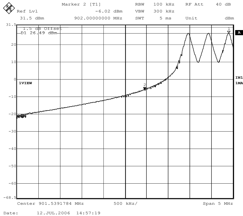
Figure 53. Band edge compliance; ISO 18000-6B mode; Channel 1, hopping enabled.
