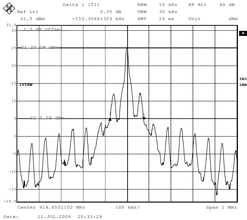
Figure 11. 20 dB Bandwidth, EPC Class 1, Channel 26.
