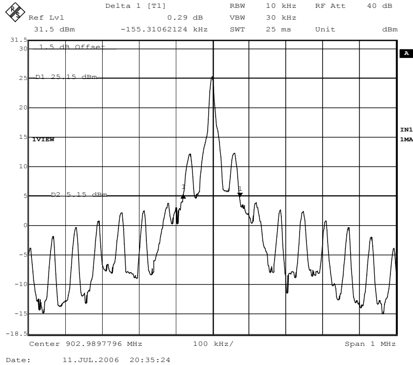
Figure 10. 20 dB Bandwidth, EPC Class 1, Channel 1.
