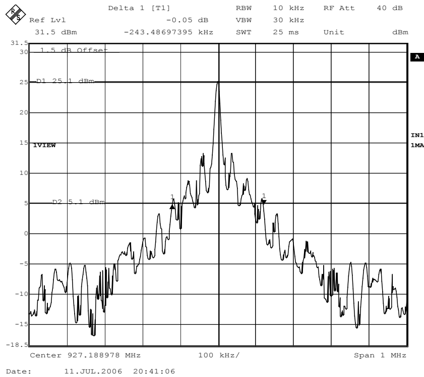
Figure 9. 20 dB Bandwidth, EPC Class 0, Channel 53.
