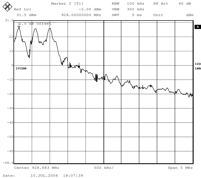
Figure 43. Band edge compliance; EPC Gen2 mode; Channel 53, hopping enabled.
