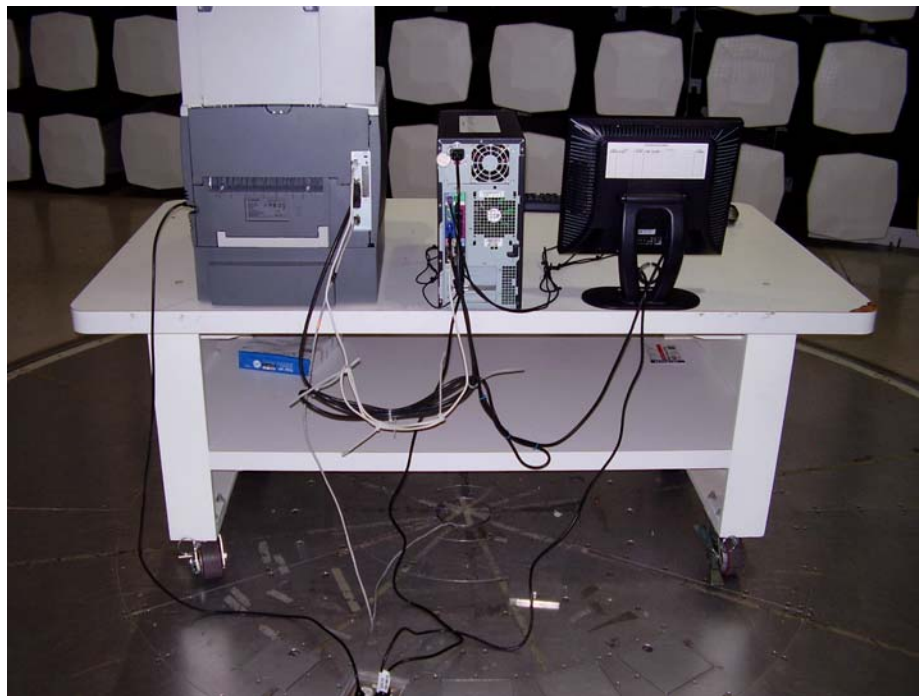
Test configuration for transmitter radiated spurious emissions (back view).
