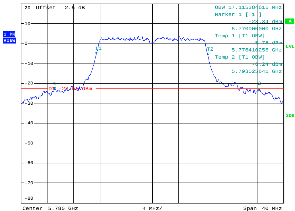
* RBW 300 kHz Delta 2 [T1 ] * VBW 1 MHz 0.14 dB SWT 20 ms 31.282051282 MHz
