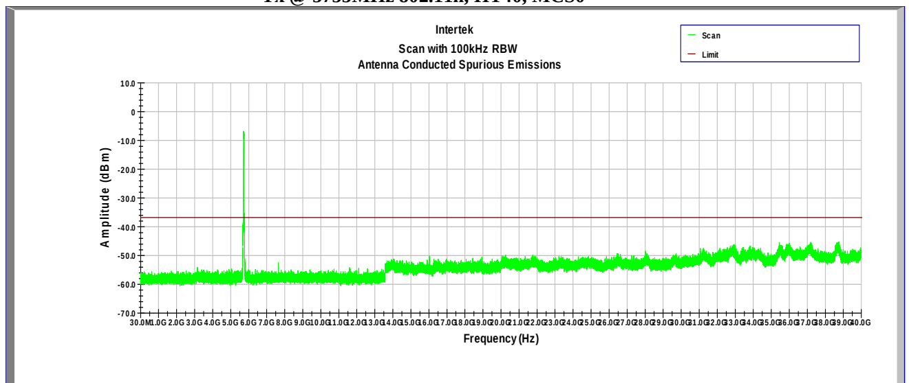
Plot 4.2 Tx @ 5755MHz 802.11n, HT40, MCS0
