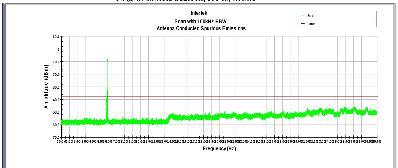
Plot 4.4 Tx @ 5795MHz 802.11n, HT40, MCS0
