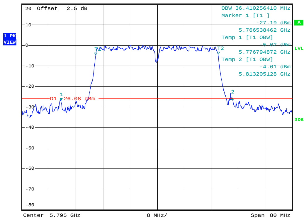
* RBW 300 kHz Delta 2 [T1 ] * VBW 500 kHz 1.21 dB SWT 20 ms 50.769230769 MHz
