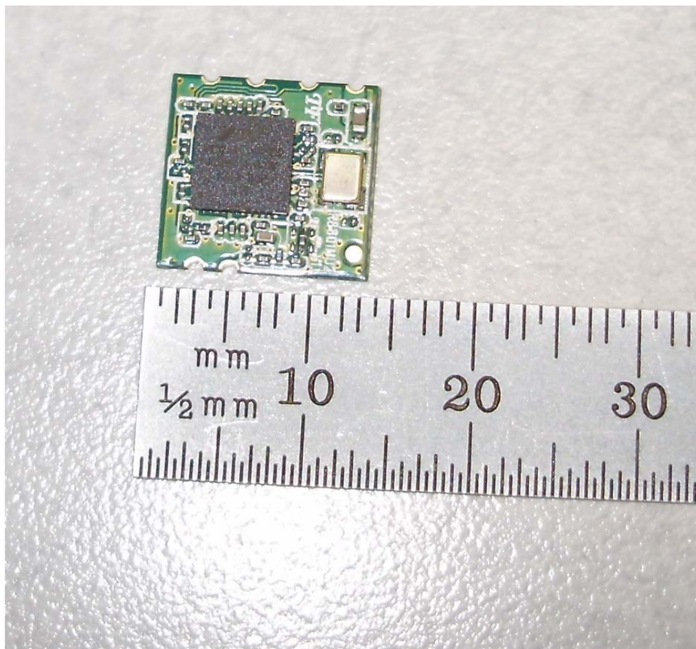
Photo 1 - LEX-M08-001 Module External Top View – shown without label
