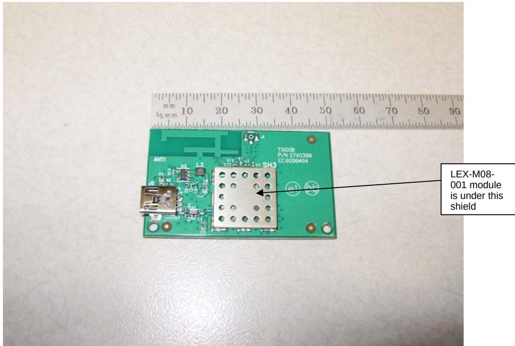
Photo 6 showing LEX-M08-001 module on host PCB under a shield.
