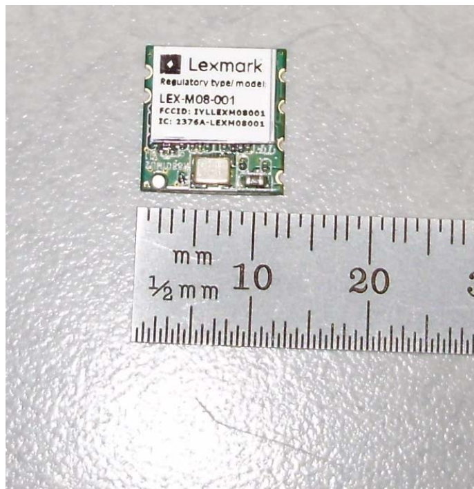
Photo 1 – LEX-M08-001 Module External Top View – shown with label
