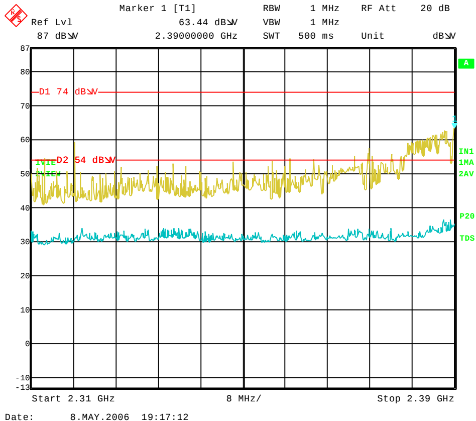
Figure 12. Radiated spurious emissions; Channel 1, 11 Mbps, horizontal polarization.
