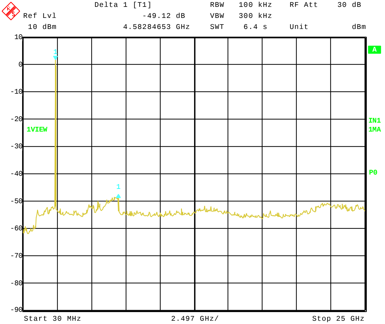
Figure 6. Out of band emissions at antenna port; Channel 1, 24 Mbps.
