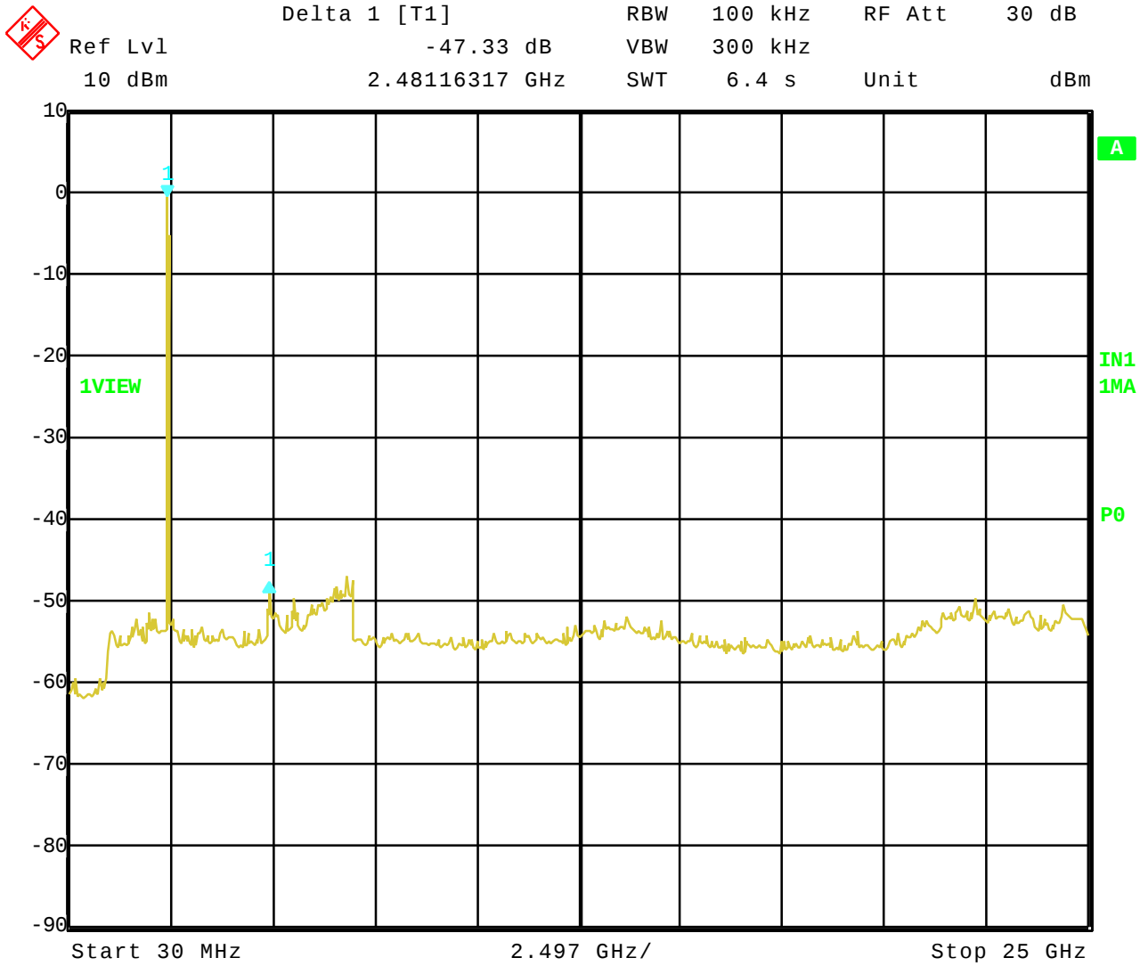
Figure 9. Out of band emissions at antenna port; Channel 11, 1 Mbps.
