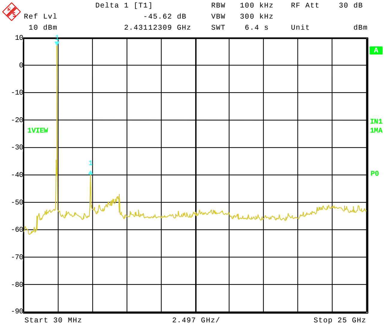
Figure 7. Out of band emissions at antenna port; Channel 6, 1 Mbps.
