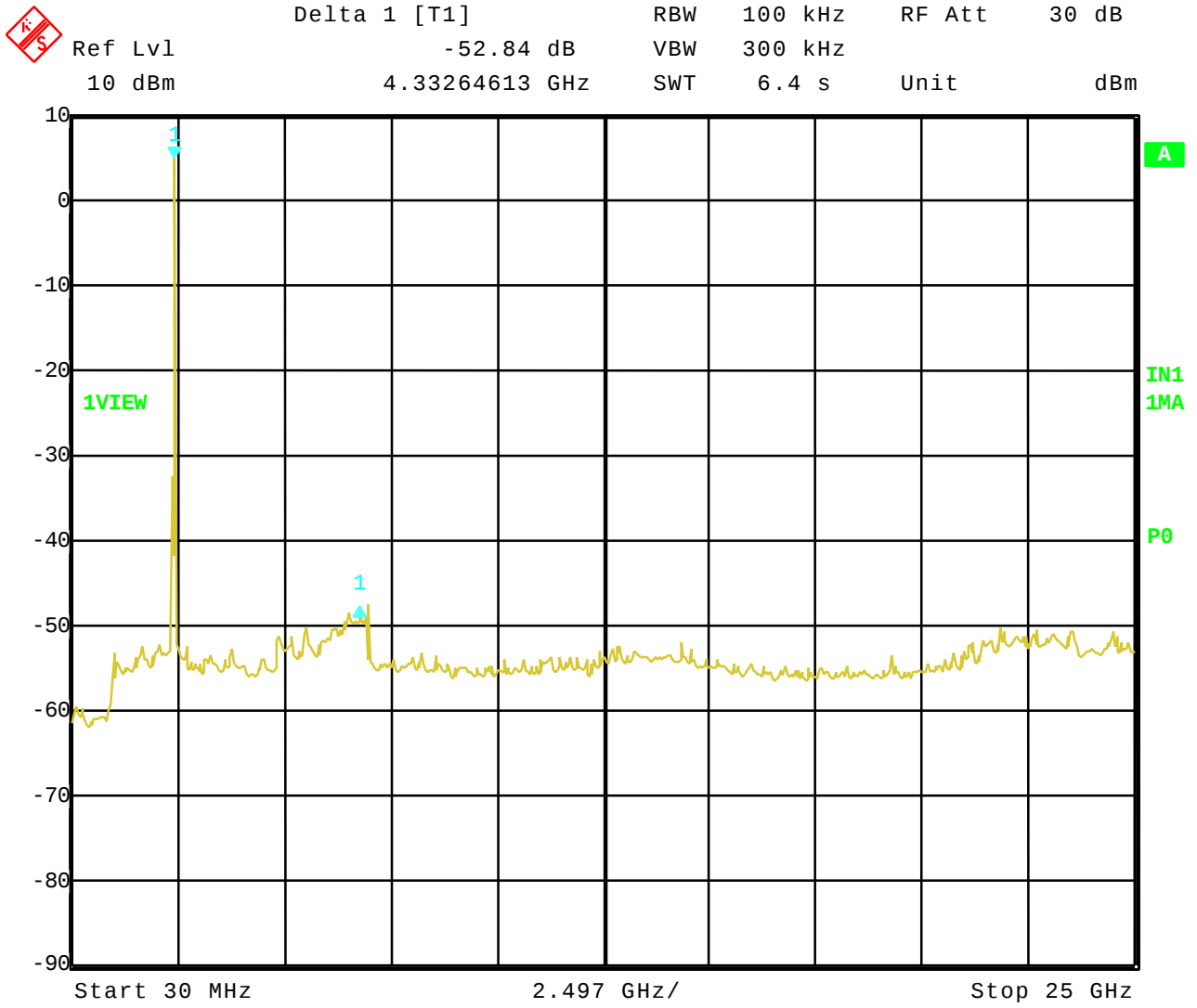
Figure 8. Out of band emissions at antenna port; Channel 6, 12 Mbps.
