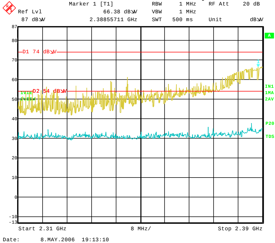
Figure 11. Radiated spurious emissions; Channel 1, 11 Mbps, vertical polarization.
