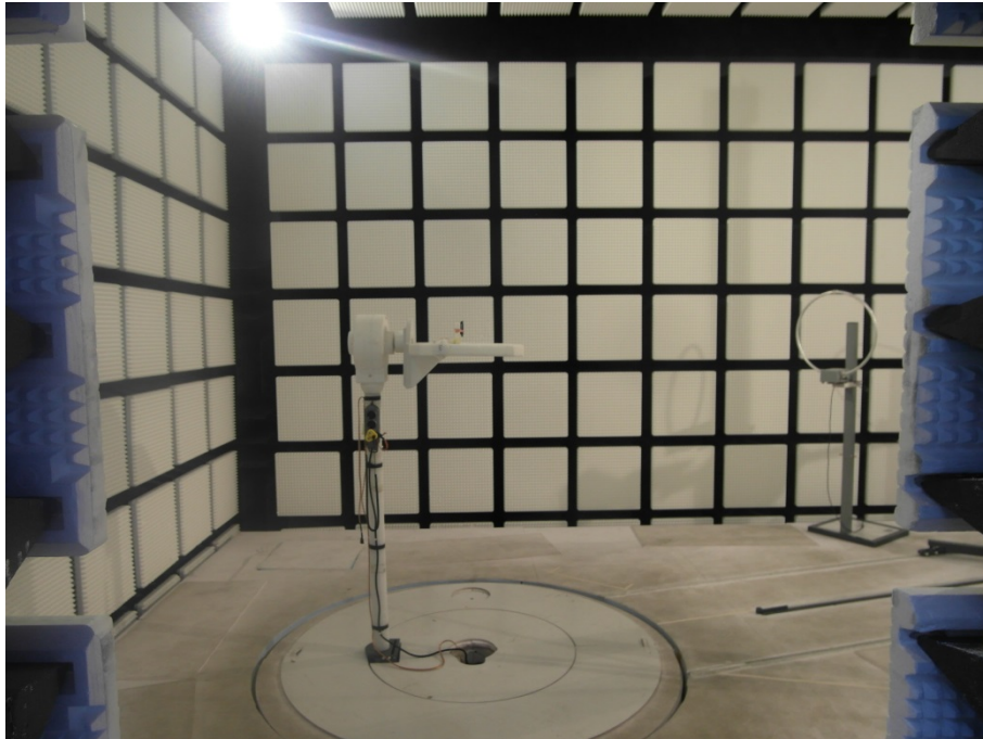
Photo 1: Setup for 1 GHz to 6 GHz
