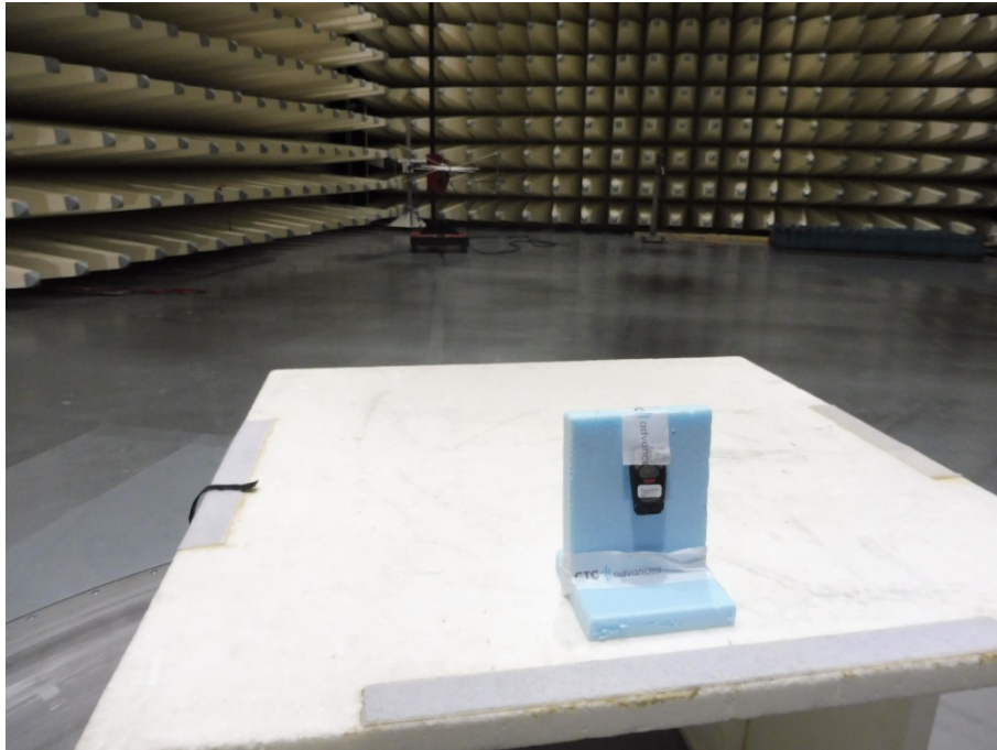
Photo 5: Setup for 30 MHz to 1 GHz
