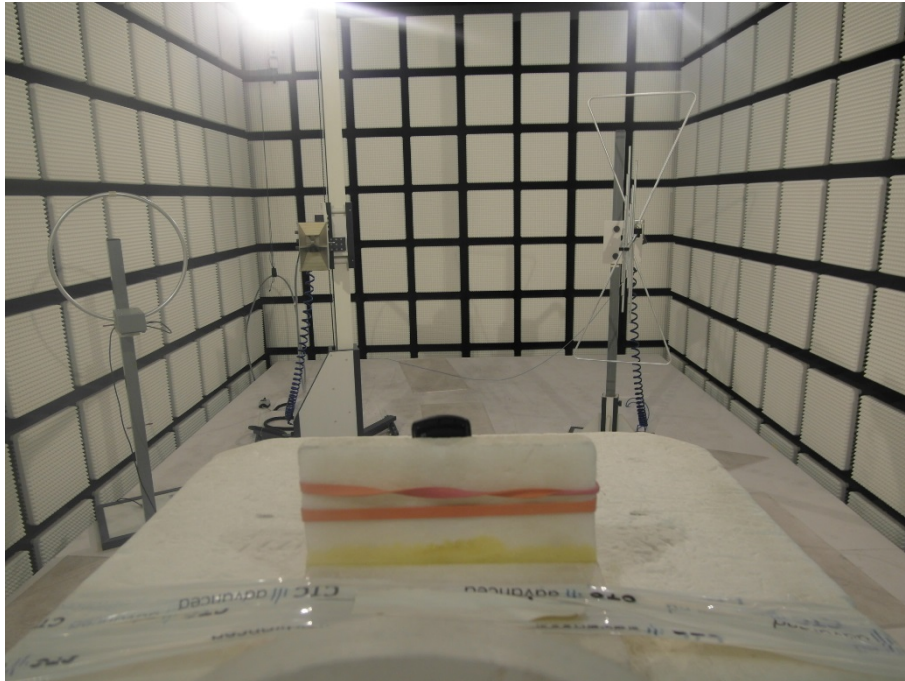
Photo 3: Setup for 1 GHz to 6 GHz
