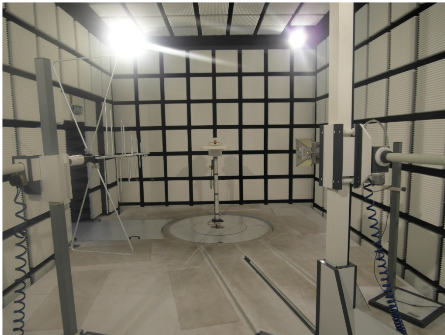
Photo 4: Setup for 1 GHz to 6 GHz
