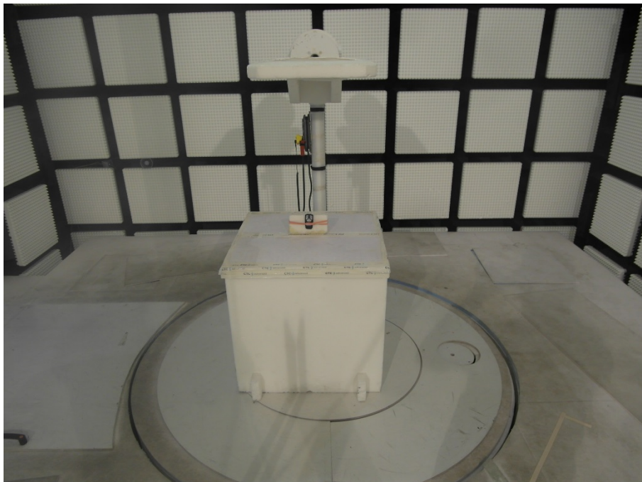
Photo 6: Setup for 9 kHz to 30 MHz
