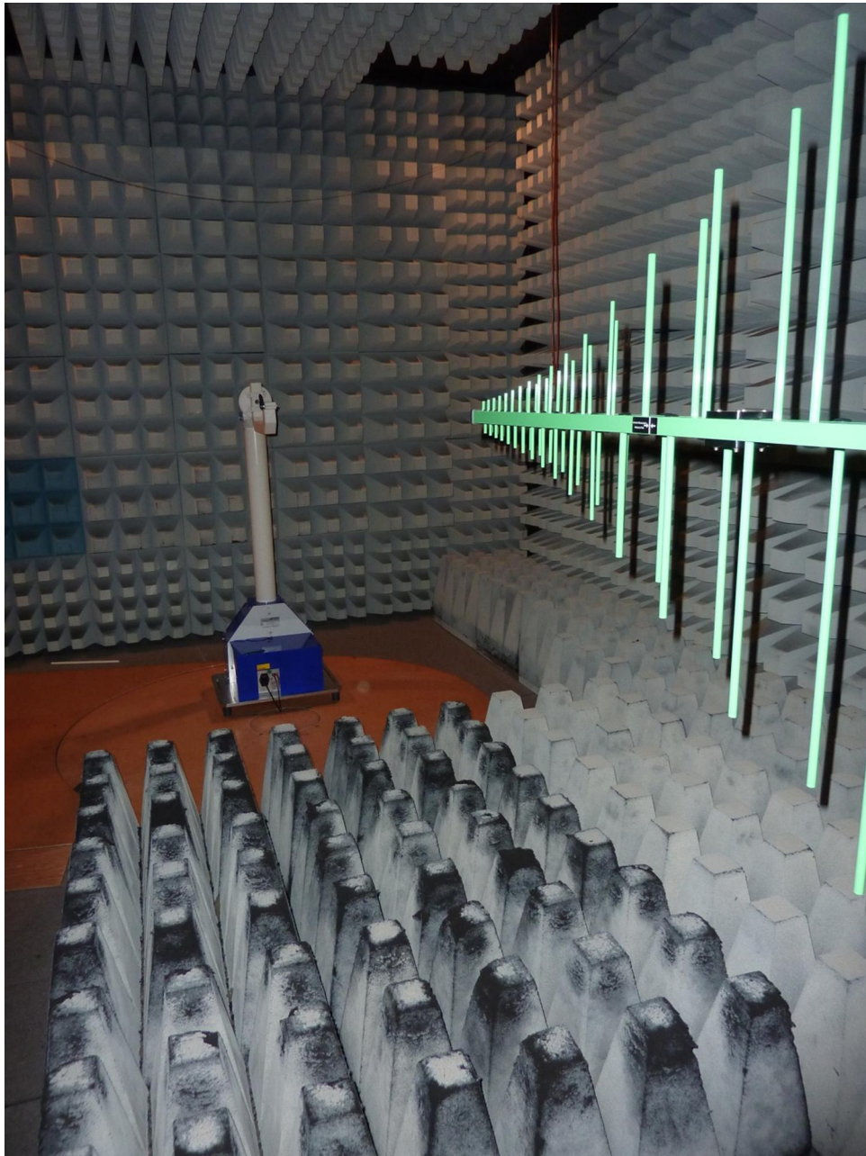
161842_2.JPG: Test setup fully anechoic chamber
