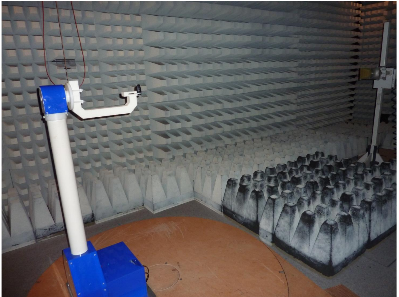
161842_3.JPG: Test setup fully anechoic chamber
