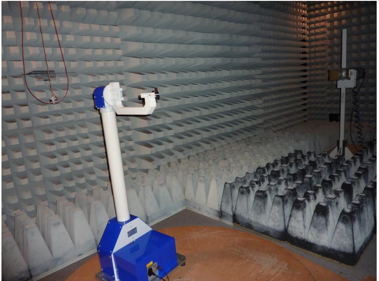
153783_13.JPG: Test setup fully anechoic chamber
