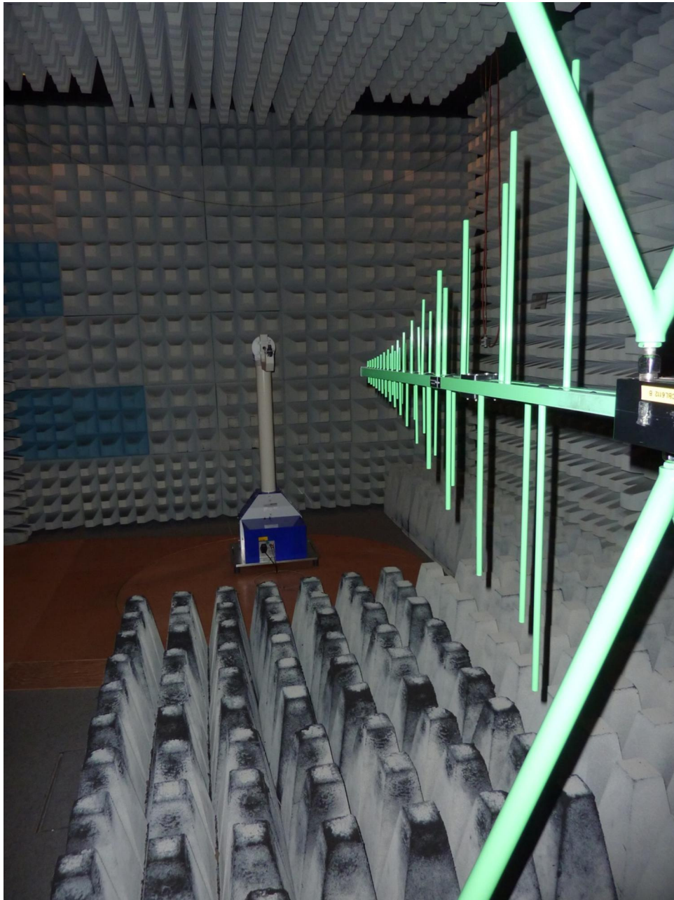
153783_2.JPG: Test setup fully anechoic chamber
