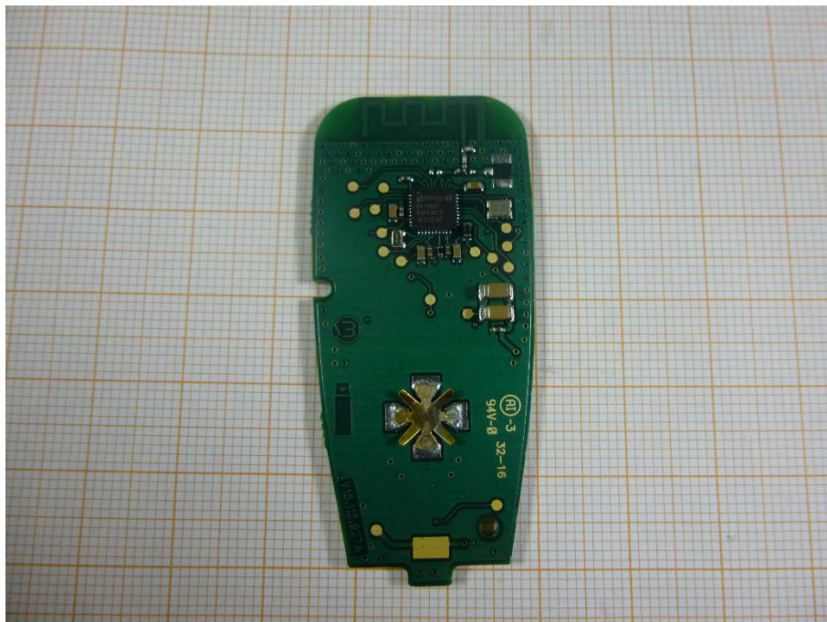
Photo 4: PCB front side view
