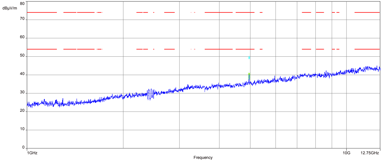
Plot 7: 1 GHz to 12.75 GHz, TX mode, 2480 MHz, vertical & horizontal polarization
