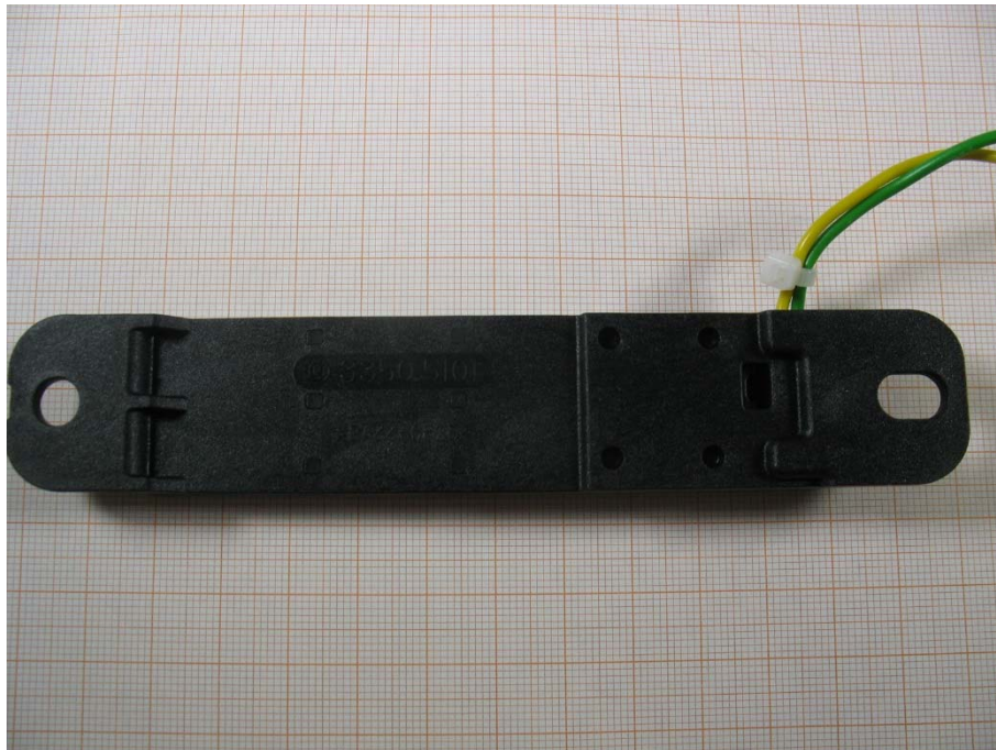
Photo 12: Test transceiver
