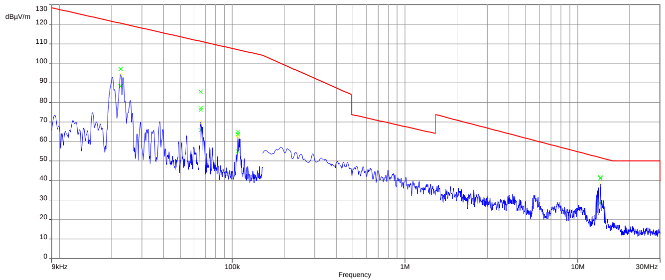
Plot 2: 9 kHz – 30 MHz, magnetic emissions, ANT 90°
