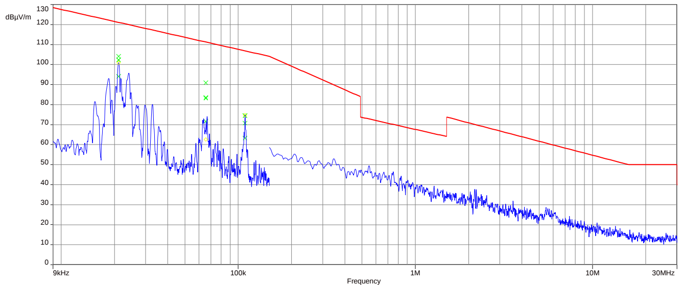
Plot 1: 9 kHz – 30 MHz, magnetic emissions, ANT 0°
