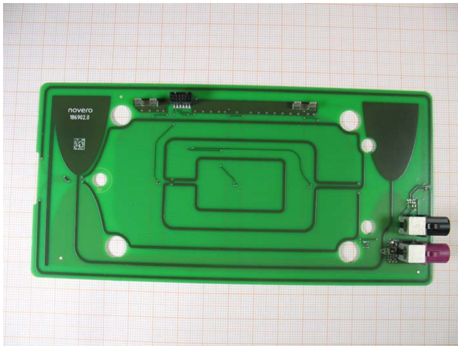
Photo 8: NFC+WPC antenna
