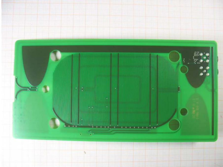
Photo 9: NFC+WPC antenna
