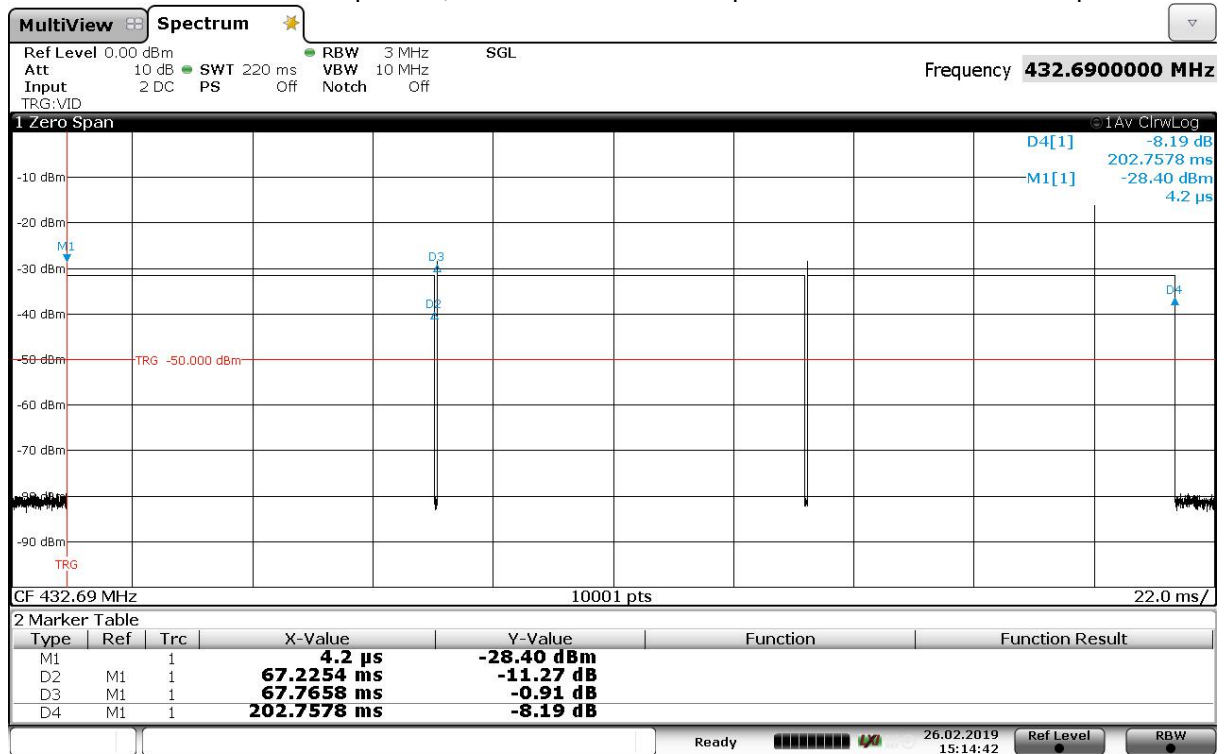
Plot 3. The 3-channel sequence, transmitted as a "triplet" after some button is pressed.
