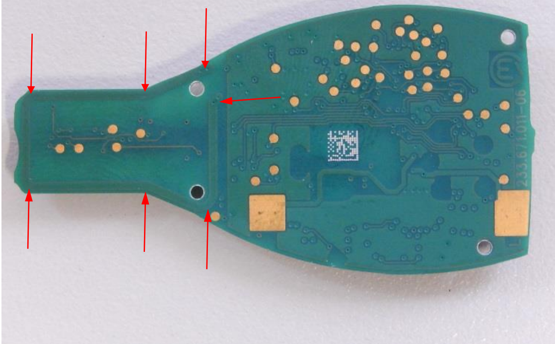
PCB Loop antenna, see marked trace
