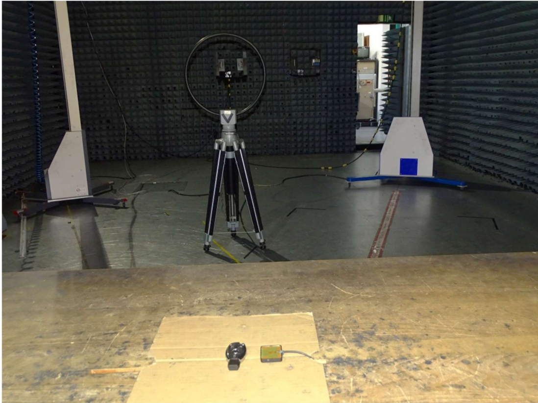
Photo 1: Test setup for radiated measurements below 30 MHz
