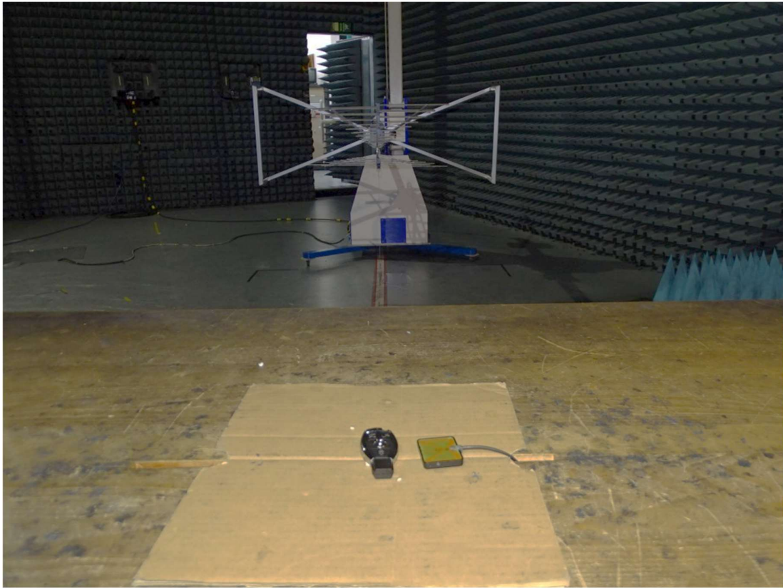
Photo 2: Test setup for radiated measurements below 1 GHz
