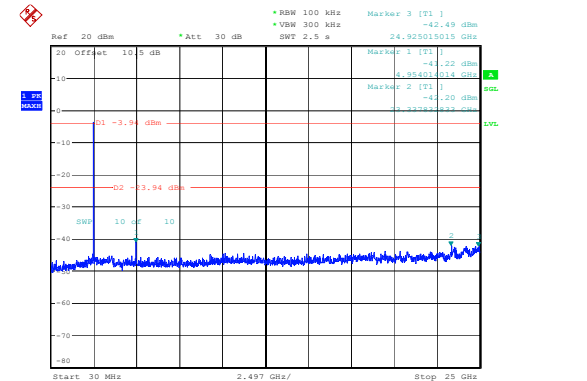
BLE_2M_High_Channel
