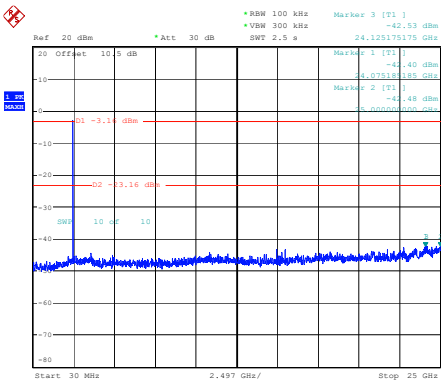
BLE_2M_Middle_Channel
