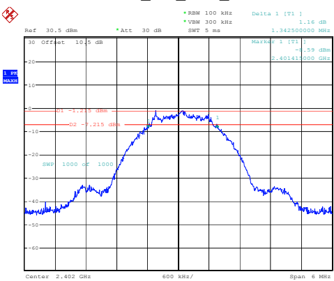
BLE_2M_Low_Channel
