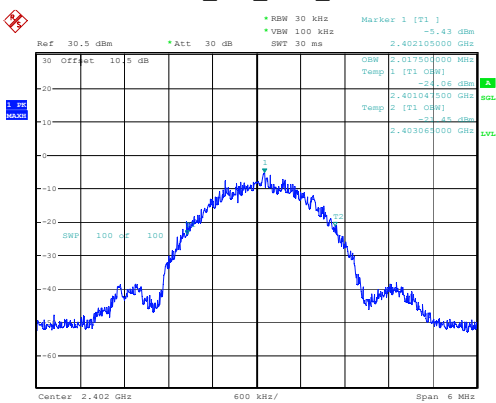
BLE_2M_Low_Channel
