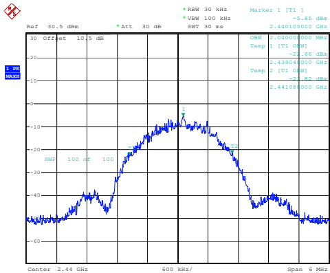
BLE_2M_Middle_Channel
