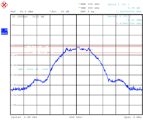
BLE_2M_High_Channel
