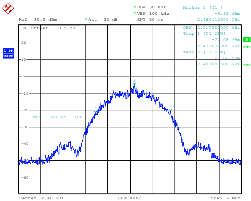
BLE_2M_High_Channel
