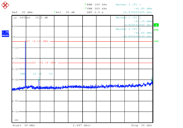
BLE_2M_Low_Channel
