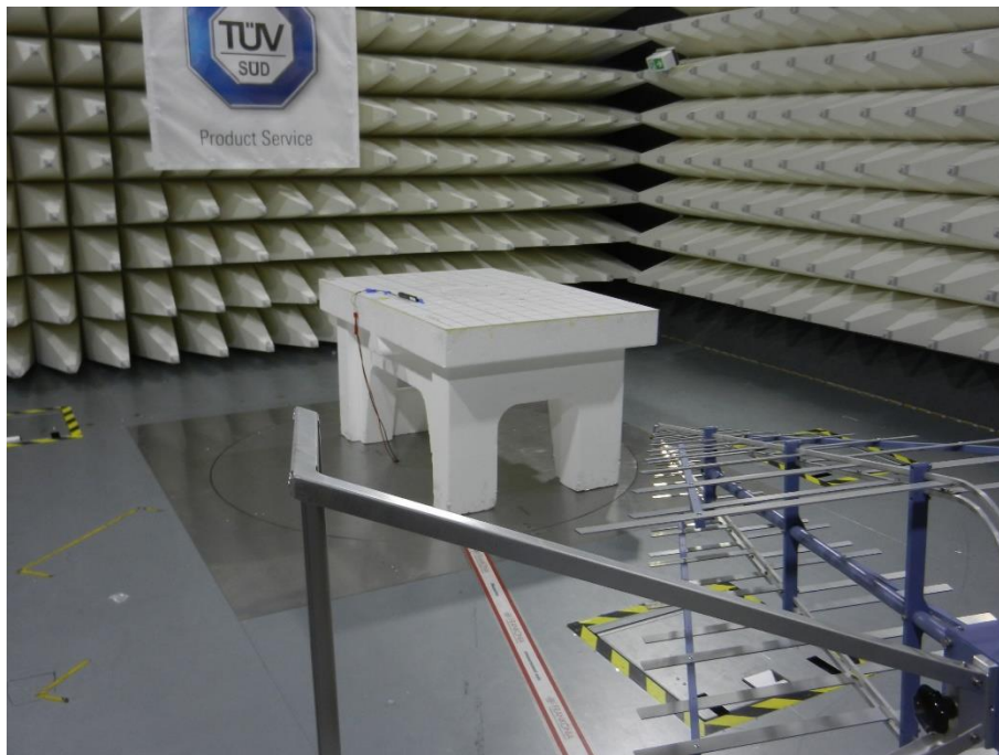
Test setup frequency range 30 MHz – 1 GHz
