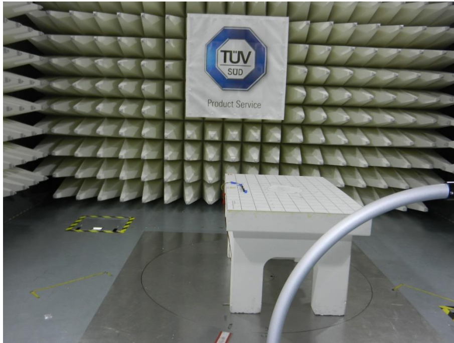
Test setup frequency range 9 kHz – 30 MHz
