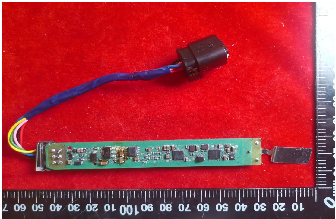
Figure 1. Top View
