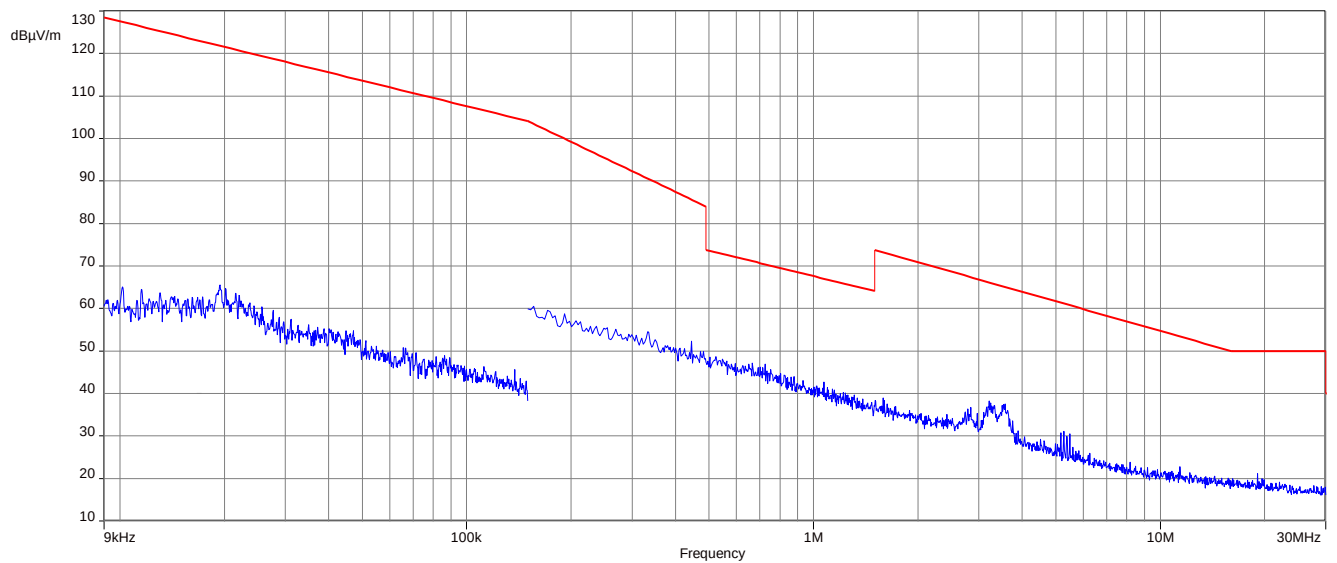
Plot 9: Channel C, 9 kHz to 30 MHz
