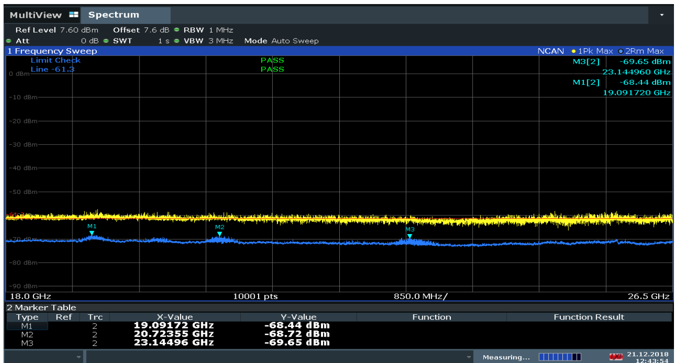
Plot 22: Max Hold on Channel A, B and C, 18 GHz to 26.5 GHz
