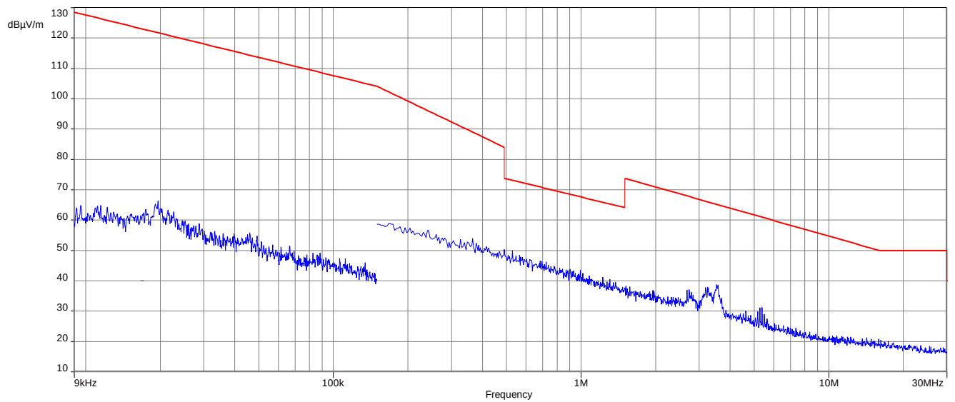
Plot 8: Channel B, 9 kHz to 30 MHz
