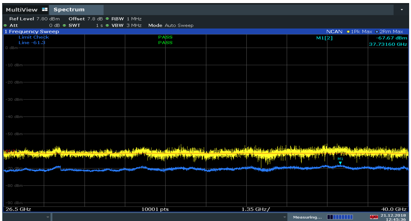
Plot 23: Max Hold on Channel A, B and C, 26.5 GHz to 40.0 GHz
